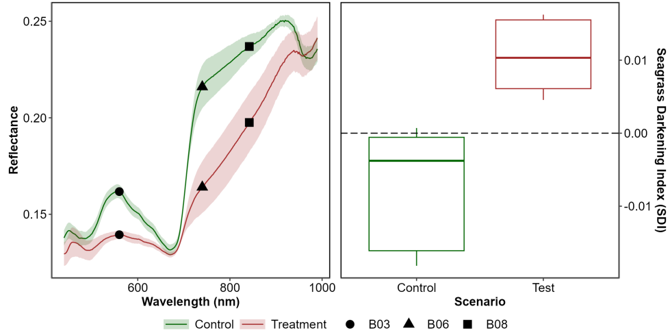
Figure 6: Development and Application of the Seagrass Darkening Index (SDI). The left panel displays the average reflectance values for both the Control and Treatment groups on the final day of the experiment. Shaded areas represent the standard deviation of reflectance, while markers indicate the spectral bands used to construct the SDI. The right panel shows the application of the SDI for both groups on the last day of the experiment.
