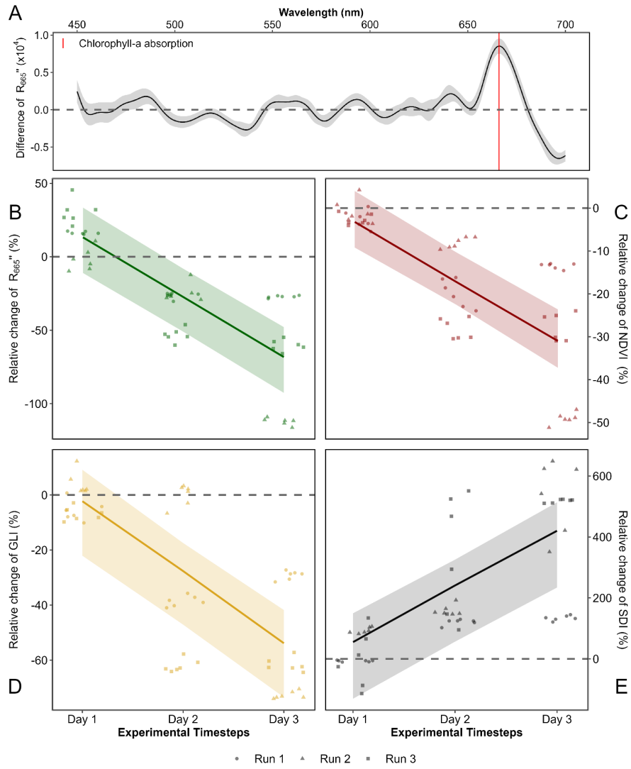
Figure 5: Difference in the second derivative of hyperspectral signature between the control and the test at the end of the experiment (A) the second derivative at 665 nm (B), the NDVI (C), the GLI (D) and the SDI (E) over Time. A: Mean difference and standard deviation of the second derivative of the Control and the Treatment on the final day of the experiment; B: Relative evolution of the second derivative at 665 nm between Treatment and Control groups over time across three replicates; C: Relative evolution of NDVI for the Treatment group compared to the Control group over time across three replicates; D: Relative evolution of GLI for the Treatment group relative to the Control group over time across three replicates; E: Relative evolution of SDI for the Treatment group relative to the Control group over time across three replicates. Points indicate raw data, the line represents a generalized linear model, and the shaded area the model's standard error.
