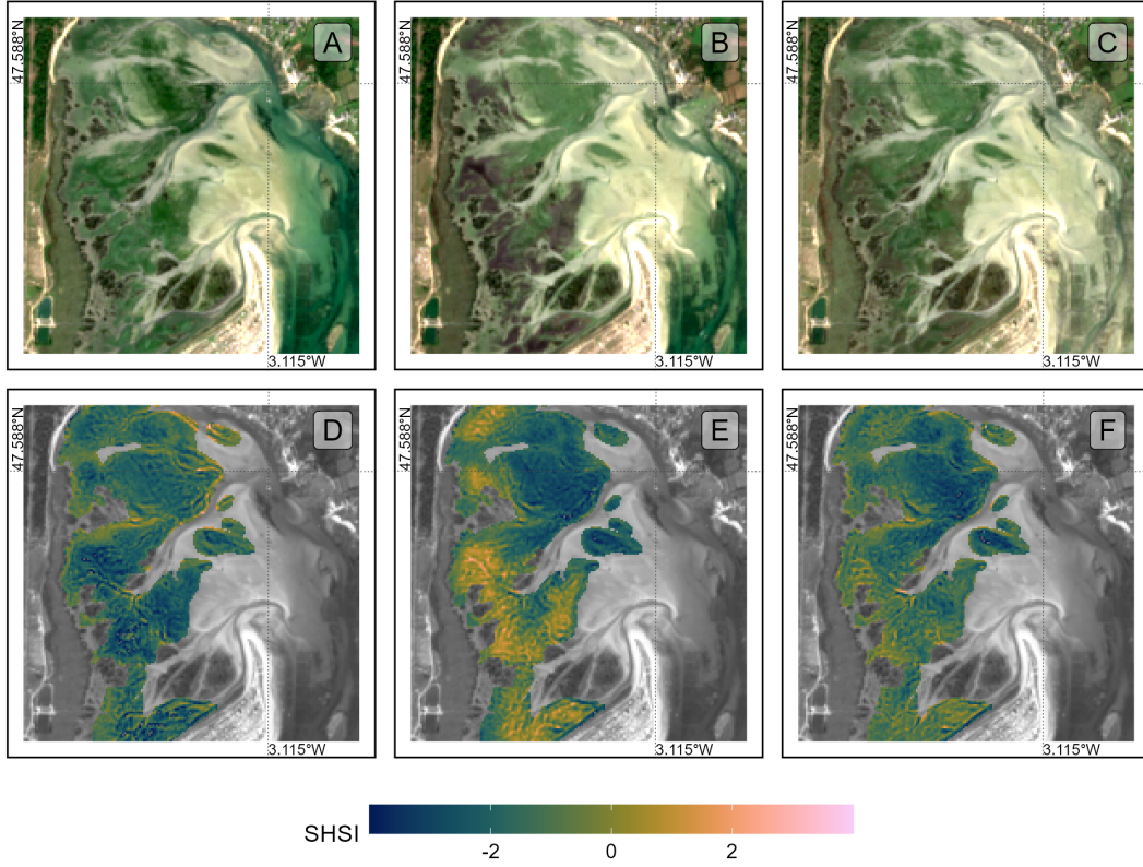
Figure 11: Sentinel-2 color composition of the seagrass meadow of Quiberon, South Brittany, France, Before (A), During (B) and After (C) the HW and SHSI applied to the same Sentinel-2 images Before (D), During (E) and After (F) the HW.
