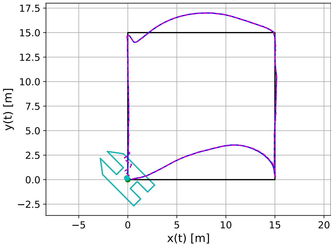
Live Plot: Current Vessel Status (real vs estimated)
