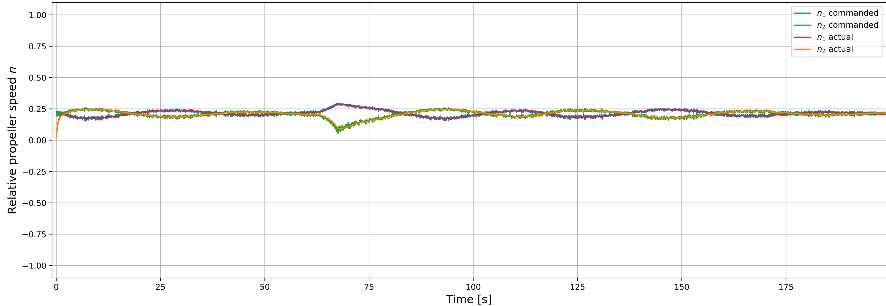
Actual vs. Commanded Propeller Speeds
