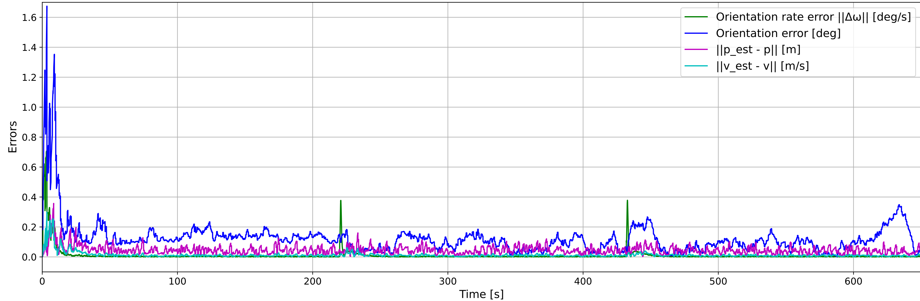
State Estimate Errors
