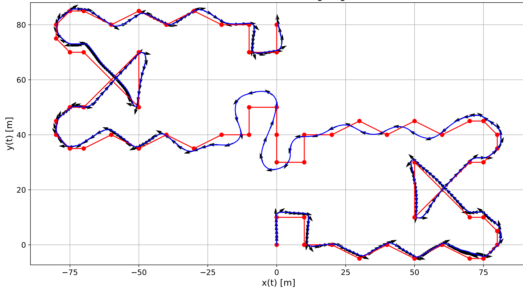
Vessel Path with Heading Angles
