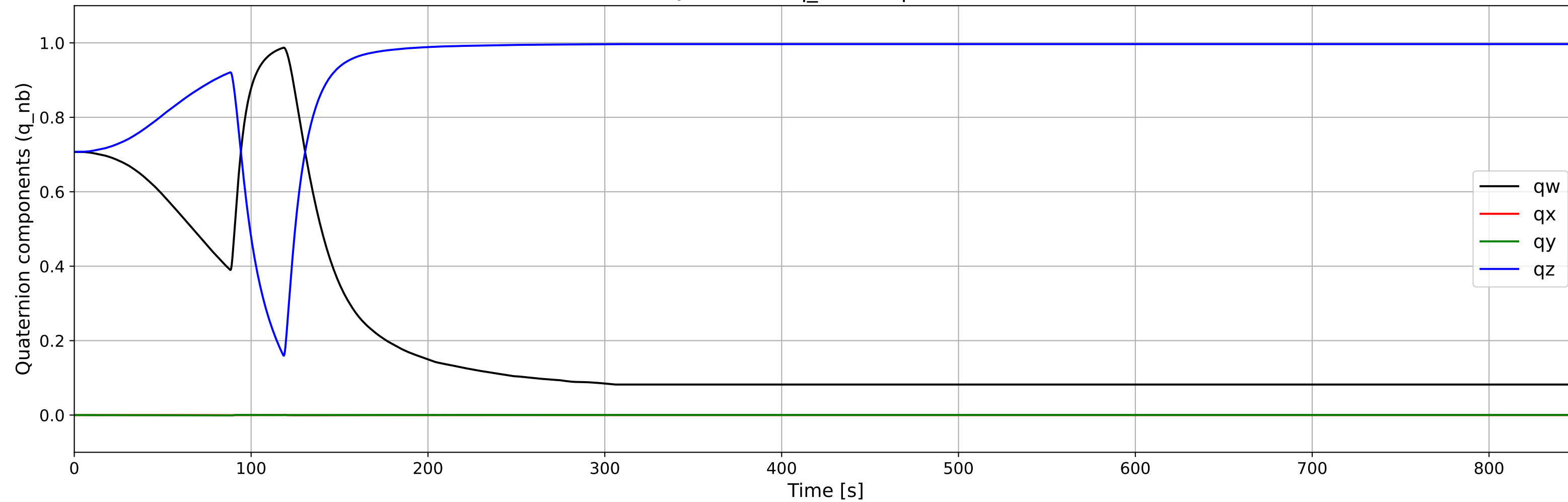
Attitude Quaternion q_{nb} Components vs Time
