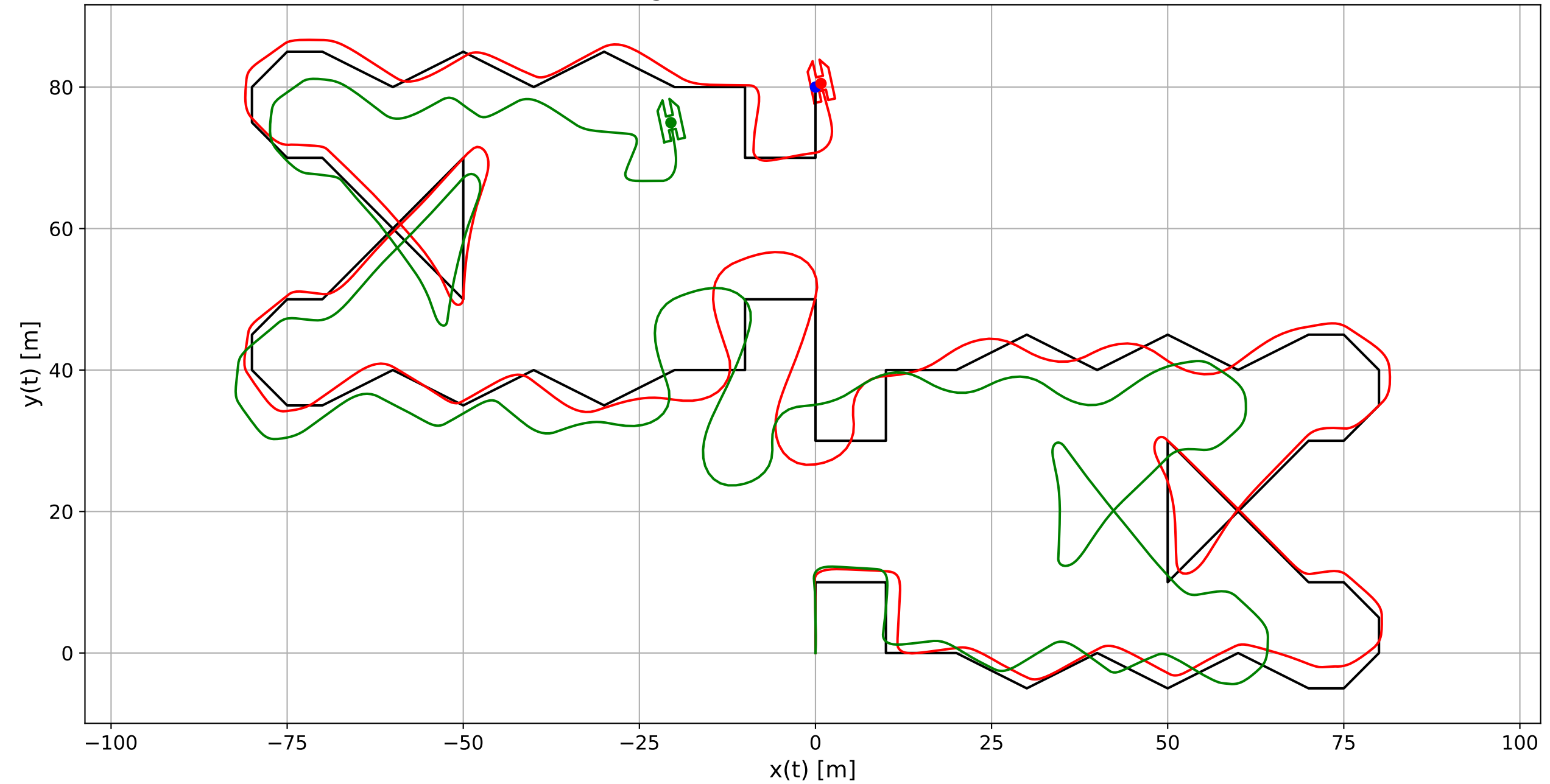
Live Plot: True (green), Estimated (red), Guidance (blue)
