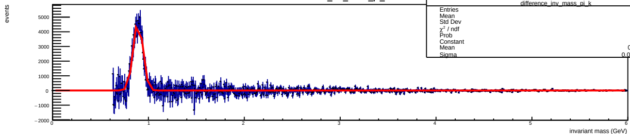
difference_inv_mass_pi_k
