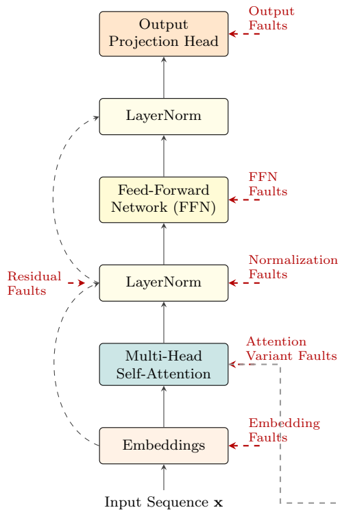
(a) Transformer Unit
