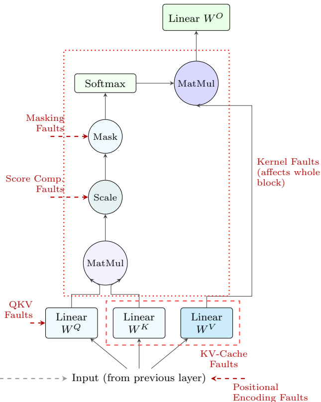
(b) Attention Internals
