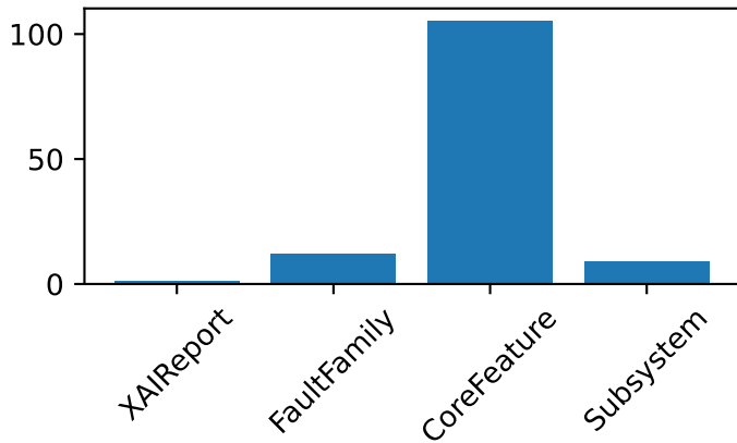
Node types
