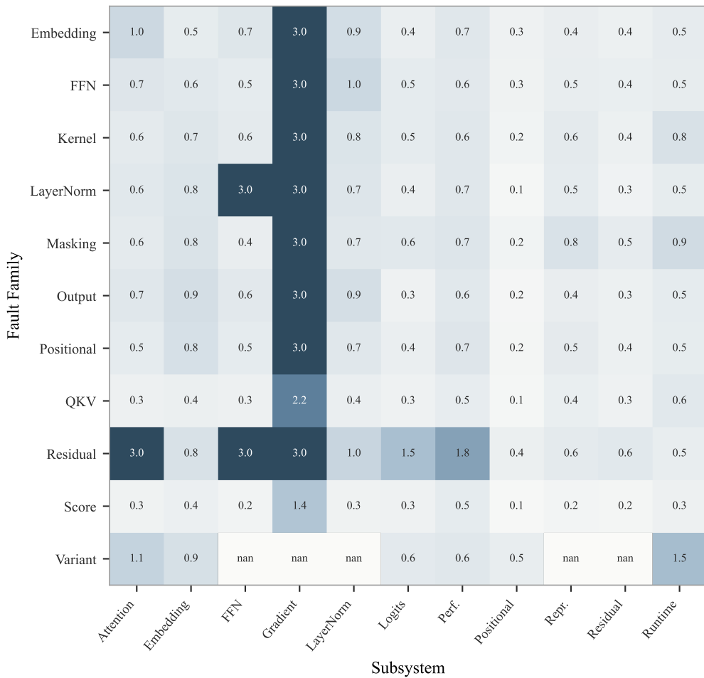
(a) Encoder
