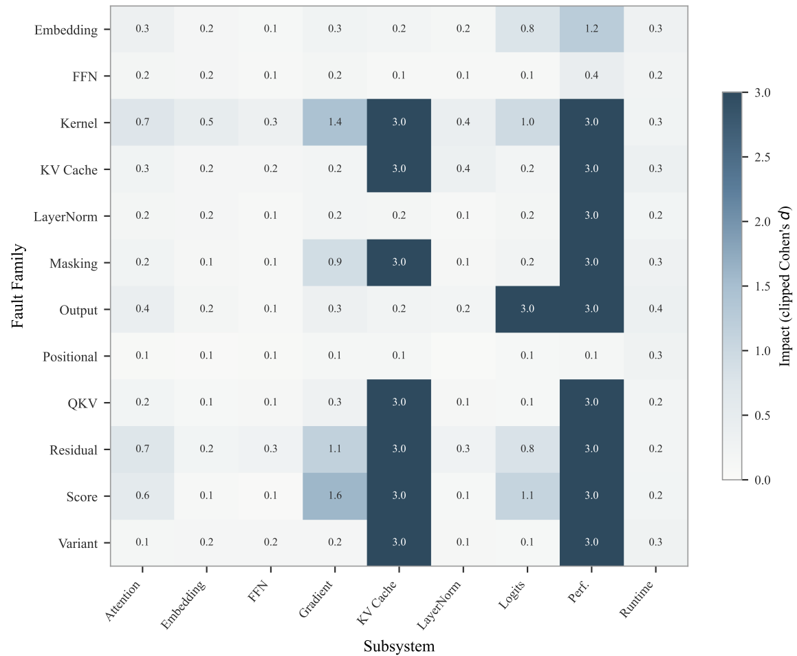
(b) Decoder
