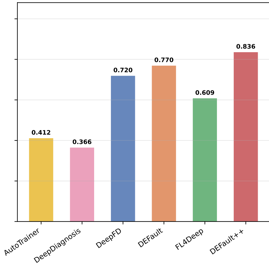
Decoder
