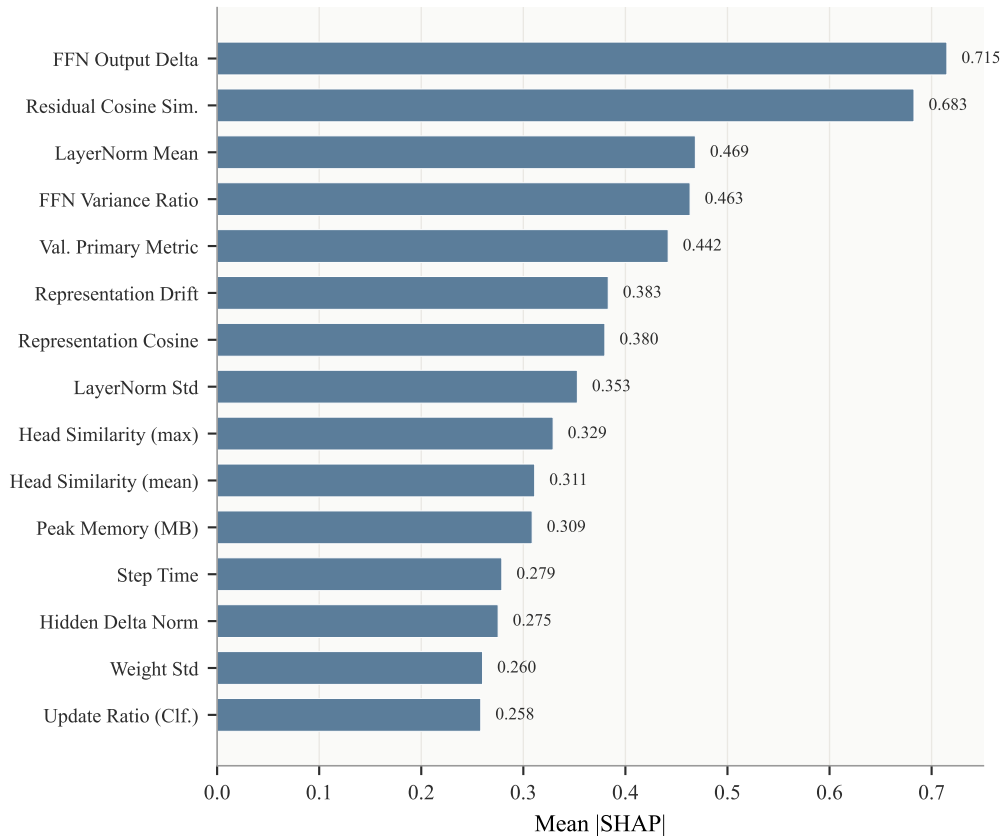
(a) Encoder
