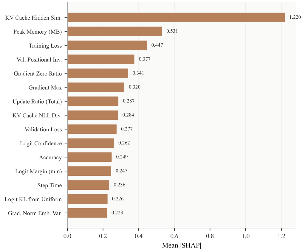
(b) Decoder
