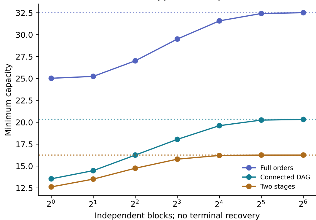
Finite horizons approach the proved limit
