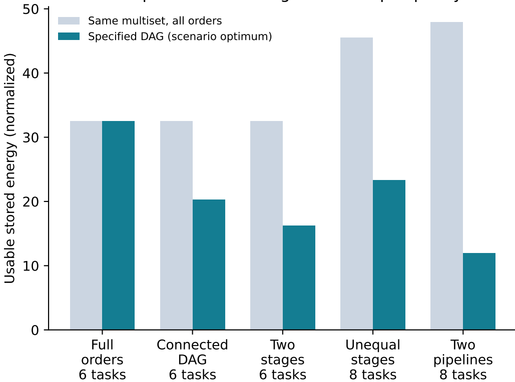
Task precedence changes the sharp capacity
