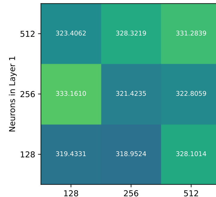
Test Loss, L3=512
