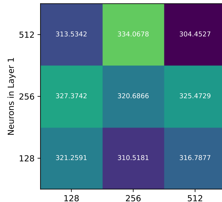
Test Loss, L3=256
