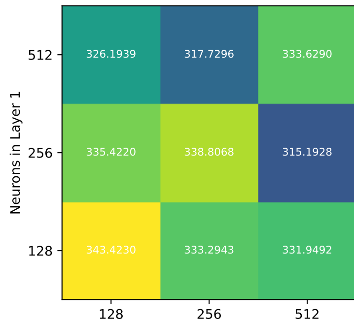
Test Loss, L3=128
