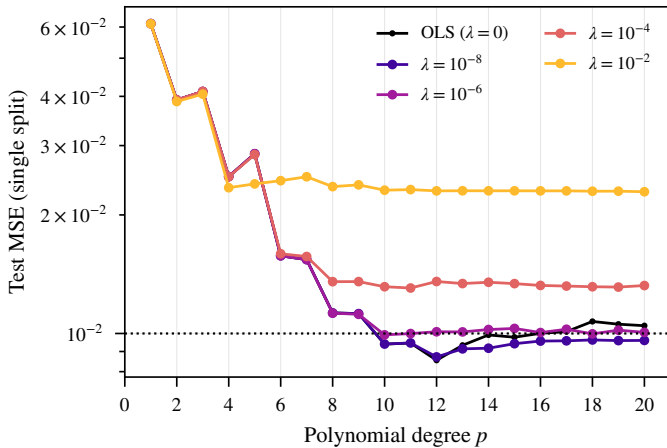
Fig. 7. Ridge test MSE vs. degree for four values of \lambda , compared with OLS (reference data set, single split). Dotted: \sigma^2 .
