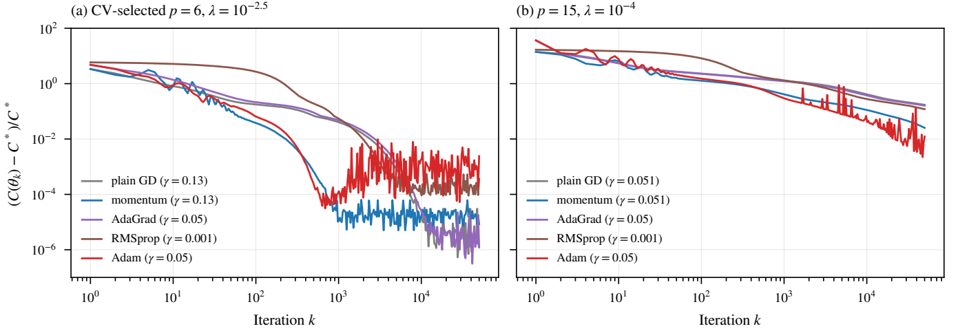
Fig. 15. Relative gap between the Lasso cost of subgradient descent and the cost C^* of scikit-learn's solution vs. iteration, from \theta = \mathbf{0} , for each update rule (reference training set). (a) The configuration selected by 5-fold CV, p = 6 , \lambda = 10^{-2.5} . (b) p = 15 , \lambda = 10^{-4} . Plain GD and momentum use \gamma = 1/L .
