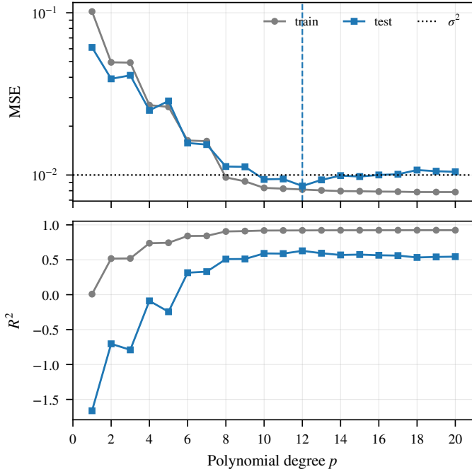
Fig. 1. OLS training and test MSE (top) and R^2 (bottom) vs. polynomial degree for the reference data set ( n = 100 , \sigma = 0.1 , 80/20 split). The dotted line is \sigma^2 ; the dashed line marks the minimum test MSE ( p = 12 ).
