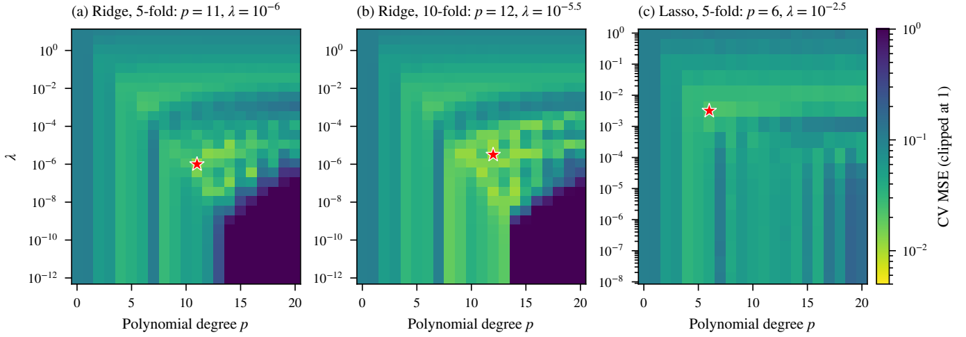
Fig. 8. CV test MSE over polynomial degree and penalty on the reference training set: Ridge with (a) 5-fold and (b) 10-fold CV, and (c) Lasso (our subgradient solver, Adam, \gamma = 0.05 , 5000 iterations) with 5-fold CV. Stars: minima. Colors are clipped at 1.
