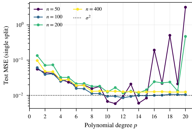
Fig. 17. OLS test MSE vs. degree for n \in \{50, 100, 200, 400\} points ( \sigma = 0.1 , 80/20 split, seed 42 for every n ).
