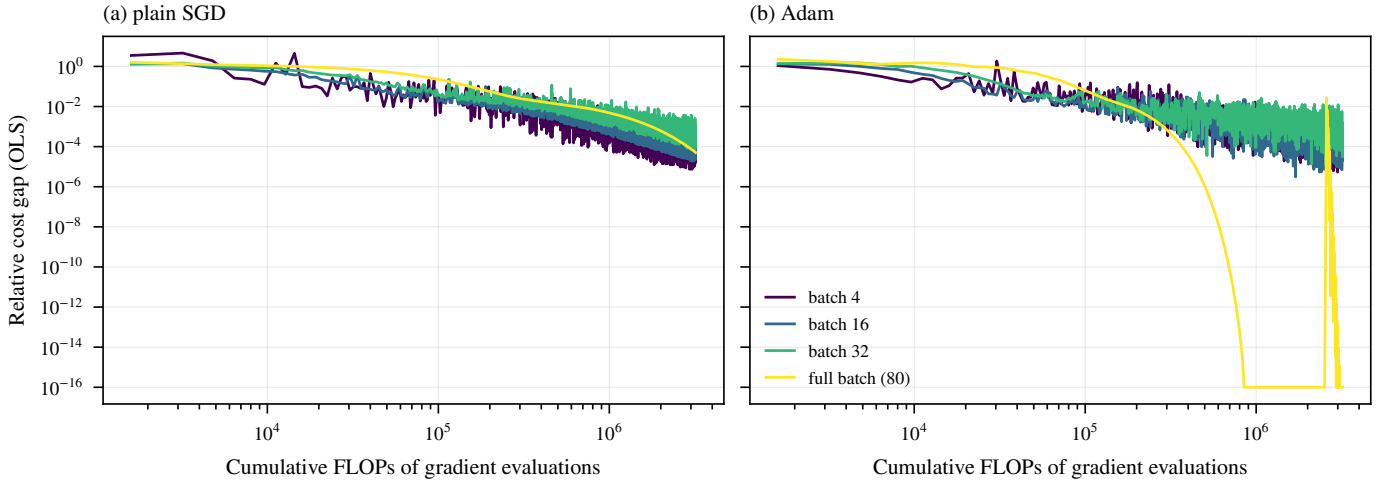
Fig. 13. Relative cost gap (OLS, p = 5 ) vs. cumulative FLOPs of the gradient evaluations for mini-batch sizes M \in \{4, 16, 32\} and the full batch ( M = 80 ), over 2000 epochs, for (a) plain SGD with \gamma_0 = 1/\lambda_{\max} and (b) Adam with \gamma_0 = 0.03 ; SGD with the decay \gamma_t = \gamma_0/(1 + 10^{-3}t) . Values below 10^{-16} are shown at 10^{-16} .
