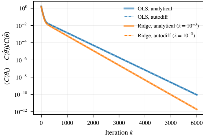
Fig. 9. Plain gradient descent with \gamma = 1/\lambda_{\max} at p = 5 (reference training set): relative gap between the cost and the cost of the closed-form solution vs. iteration, for OLS and Ridge ( \lambda = 10^{-3} ), with analytical (thick) and JAX (dashed) gradients.
