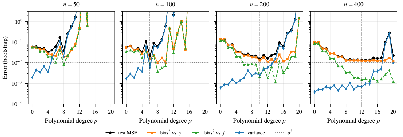
Fig. 15. Bootstrap bias–variance decomposition of the OLS test error for n \in \{50, 100, 200, 400\} at \sigma = 0.1 . Dashed: minimum of the test MSE. Values above 3 are cut off.
