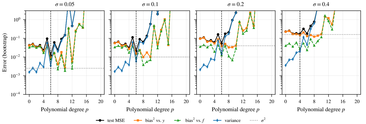
Fig. 16. Bootstrap bias–variance decomposition of the OLS test error for \sigma \in \{0.05, 0.1, 0.2, 0.4\} at n = 100 .
