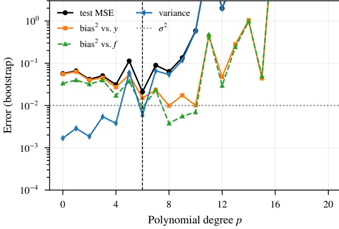
Fig. 5. Bootstrap bias-variance decomposition of the OLS test error ( B = 100 , reference data set). The squared bias is measured both against the noisy test targets y (eq. (16), absorbs \sigma^2 ) and against the true f (eq. (14)). Dashed: minimum of the bootstrap test MSE ( p = 6 ). Values above 3 are cut off.
