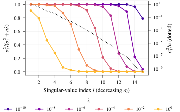
Fig. 3. Ridge shrinkage factors d_i = \sigma_i^2 / (\sigma_i^2 + n\lambda) (eq. (8)) of the SVD modes of the standardized design matrix at p = 15 (training set of the reference data), for \lambda from 10^{-10} to 1. Dotted, right axis: \sigma_i^2/n .
