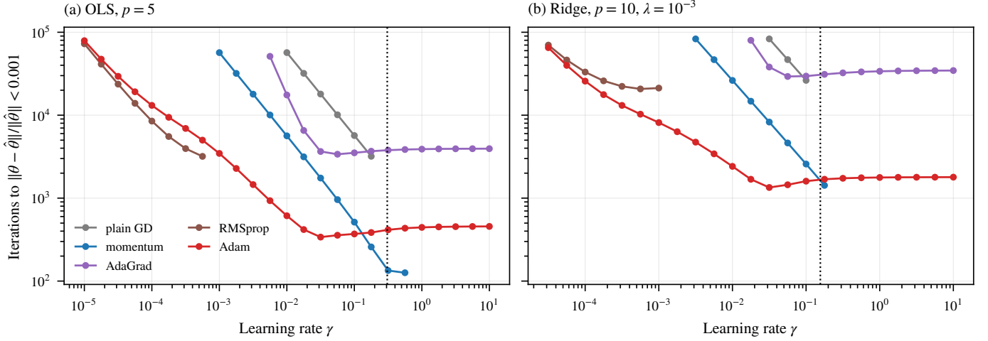
Fig. 11. Iterations to reach the closed-form solution to a relative parameter error of 10^{-3} vs. the learning rate, for each optimizer. Missing points: tolerance not reached within 10^5 iterations, or divergence. Dotted: the plain-GD stability bound 2/\lambda_{\max}(\mathbf{H}) .
