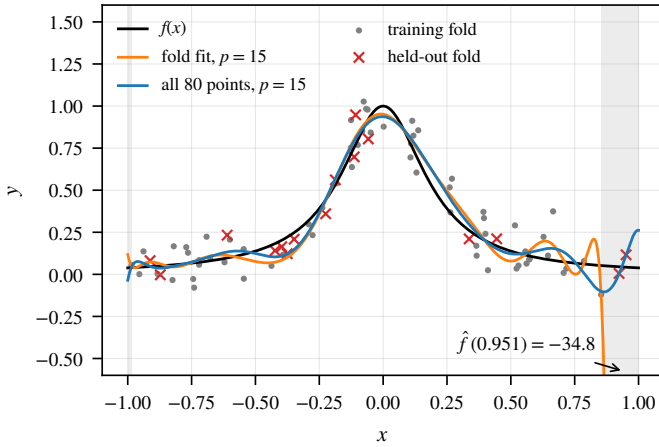
Fig. 7. The 5-fold CV split that dominates the CV estimate at p = 15 (reference data). Orange: fit on the four training folds (gray points), which must extrapolate beyond their range (shaded) to the held-out point at x = 0.951 . Blue: fit on all 80 training points.
