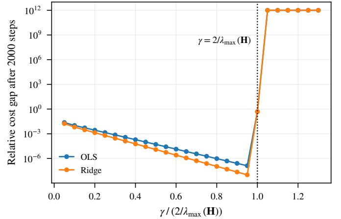
Fig. 10. Relative cost gap after 2000 plain-GD steps vs. the learning rate in units of the bound 2/\lambda_{\max}(\mathbf{H}) ( p = 5 ). Diverged runs are shown at 10^{12} .
