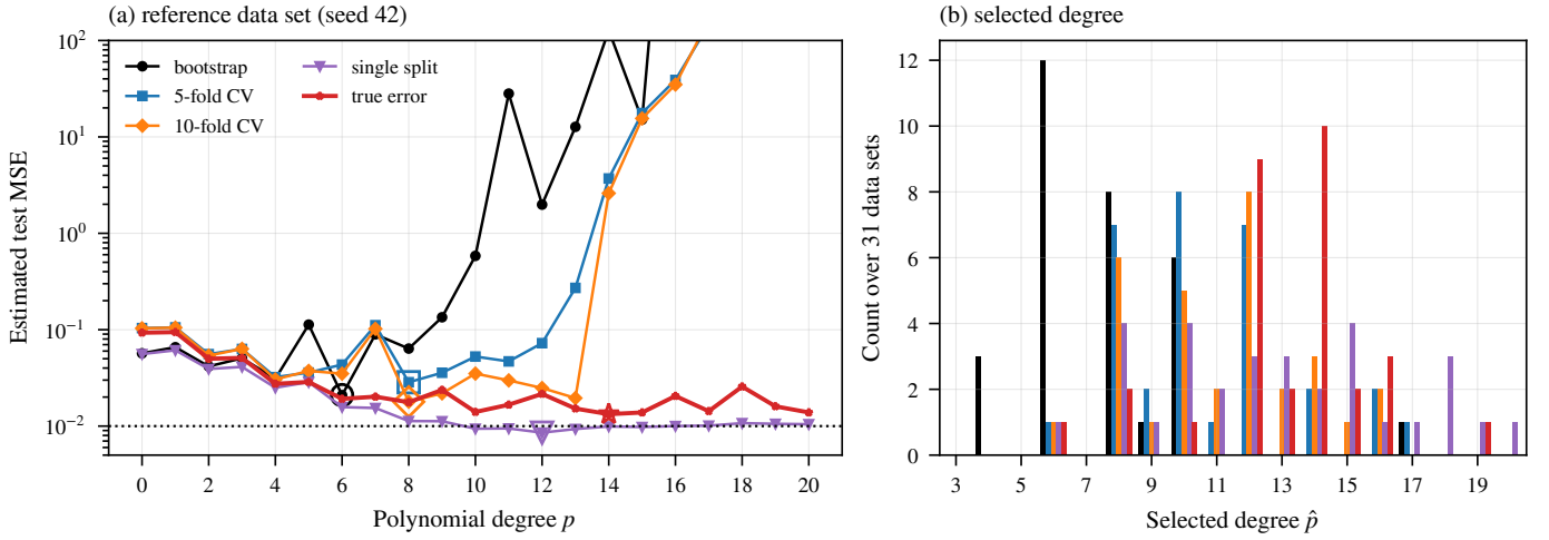
Fig. 6. Estimated OLS test error vs. degree. (a) Reference data set: bootstrap ( B = 100 ), 5- and 10-fold CV and a single 80/20 split, all computed from the same 80 training points, and the true error of the fit on those 80 points (from the known f ). Open markers: minima. (b) Degree selected by each estimator over 31 independent data sets.
