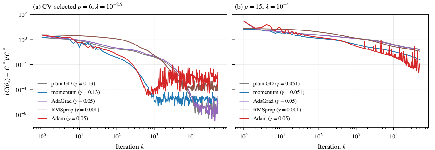
Fig. 12. Relative gap between the Lasso cost of subgradient descent and the cost C^* of scikit-learn's solution vs. iteration, from \theta = \mathbf{0} , for each update rule (reference training set). (a) The configuration selected by 5-fold CV, p = 6 , \lambda = 10^{-2.5} . (b) p = 15 , \lambda = 10^{-4} . Plain GD and momentum use \gamma = 1/\lambda_{\max} .
