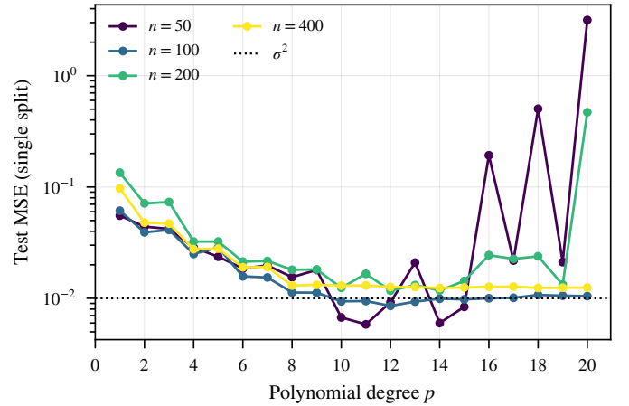
Fig. 4. OLS test MSE vs. degree for n \in \{50, 100, 200, 400\} points ( \sigma = 0.1 , 80/20 split, seed 42 for every n ).
