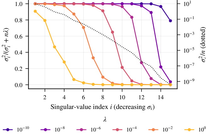
Fig. 5. Ridge shrinkage factors d_i = \sigma_i^2 / (\sigma_i^2 + n\lambda) (eq. (8)) of the SVD modes of the standardized design matrix at p = 15 (training set of the reference data), for \lambda from 10^{-10} to 1. Dotted, right axis: \sigma_i^2/n .
