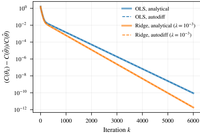
Fig. 12. Plain gradient descent with \gamma = 1/\lambda_{\max} at p = 5 (reference training set): relative gap between the cost and the cost of the closed-form solution vs. iteration, for OLS and Ridge ( \lambda = 10^{-3} ), with analytical (thick) and JAX (dashed) gradients.
