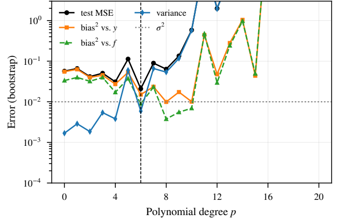
Fig. 8. Bootstrap bias-variance decomposition of the OLS test error ( B = 100 , reference data set). The squared bias is measured both against the noisy test targets \mathbf{y} (eq. (15), absorbs \sigma^2 ) and against the true \mathbf{f} (eq. (13)). Dashed: minimum of the bootstrap test MSE ( p = 6 ). Values above 3 are cut off.
