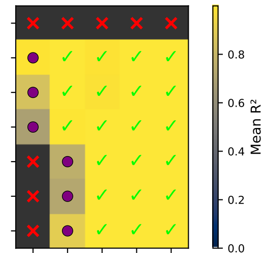
Transformer
