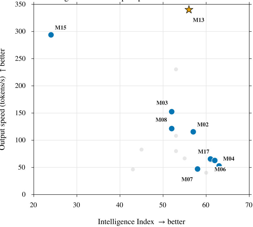
B. Intelligence versus output speed
