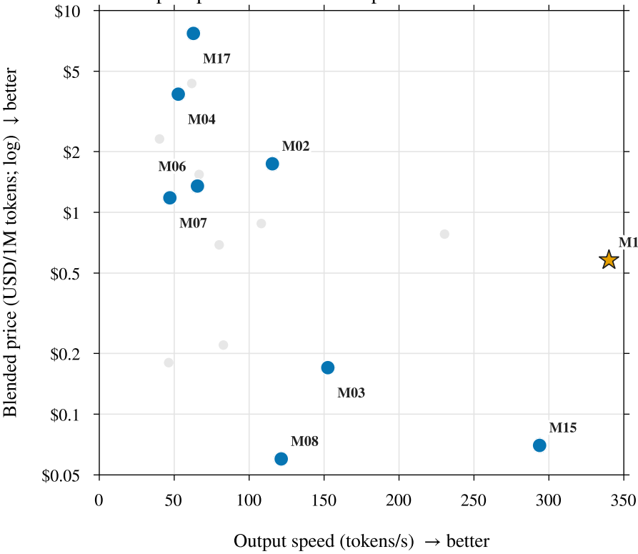
D. Output speed versus blended price
