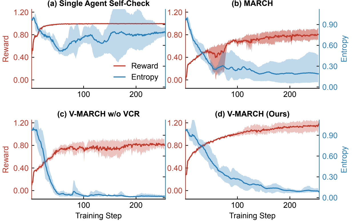
Figure 6 | Reward (red, left axis) and entropy (blue, right axis) curves over 256 training steps for (a) Single Agent SelfCheck, (b) MARCH (Li et al., 2026), (c) V-MARCH w/o VCR, and (d) V-MARCH . The comparison demonstrates that claim-level verification with VCR is necessary for stable, non-degenerate training.
