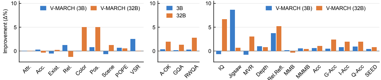
Figure 5 | Per-metric performance improvements ( \Delta\% ) of V-MARCH over the respective Qwen2.5-VL-3B and Qwen2.5-VL-32B base models, across (a) Hallucination, (b) Real-World VQA, and (c) Mixed Benchmarks.
