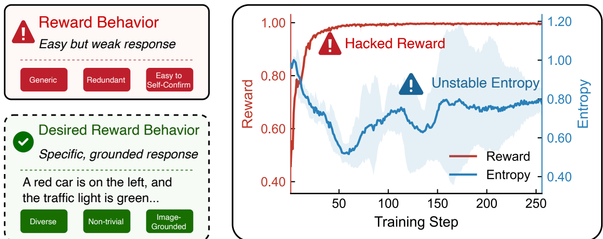
Figure 2 | Motivation. Naive self-verification rewards vague but safe descriptions, causing rapid reward growth that reflects reward hacking rather than genuine visual grounding. Reliable visual self-verification should instead favor diverse, non-trivial, and image-grounded claims while maintaining stable training.
