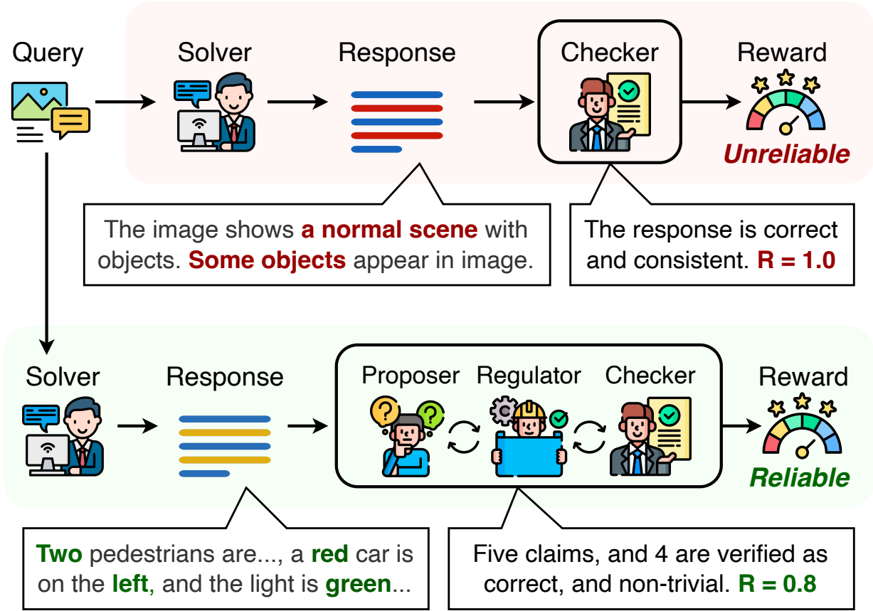
Figure 1 | V-MARCH achieves reliable visual self-verification rewards through a multi-agent self-check mechanism, encouraging VLMs to generate more informative, image-supported, and diverse responses.
