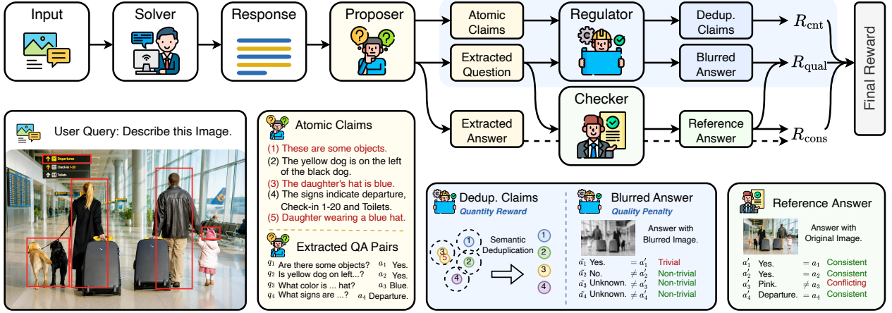
Figure 3 | Overview of the V-MARCH pipeline. Given a Solver -generated response, the Proposer decomposes it into atomic factual claims and converts each into a visual question-answer pair. The Regulator performs Visual Claim Regulation (VCR) by deduplicating semantically redundant claims, rewarding claim quantity, and penalizing image-agnostic claims that can be answered without genuine visual perception. The Checker re-answers each question using the original image, and verifies consistency with the Solver’s answers. The final self-verifying reward aggregates the Checker’s consistency signal and the Regulator’s quantity and quality signals.
