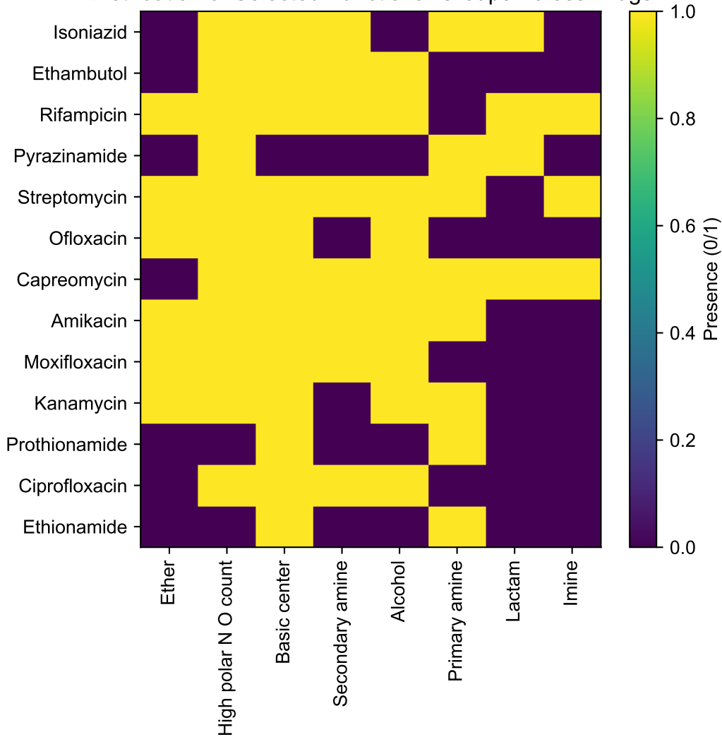
Distribution of Selected Functional Groups Across Drugs
