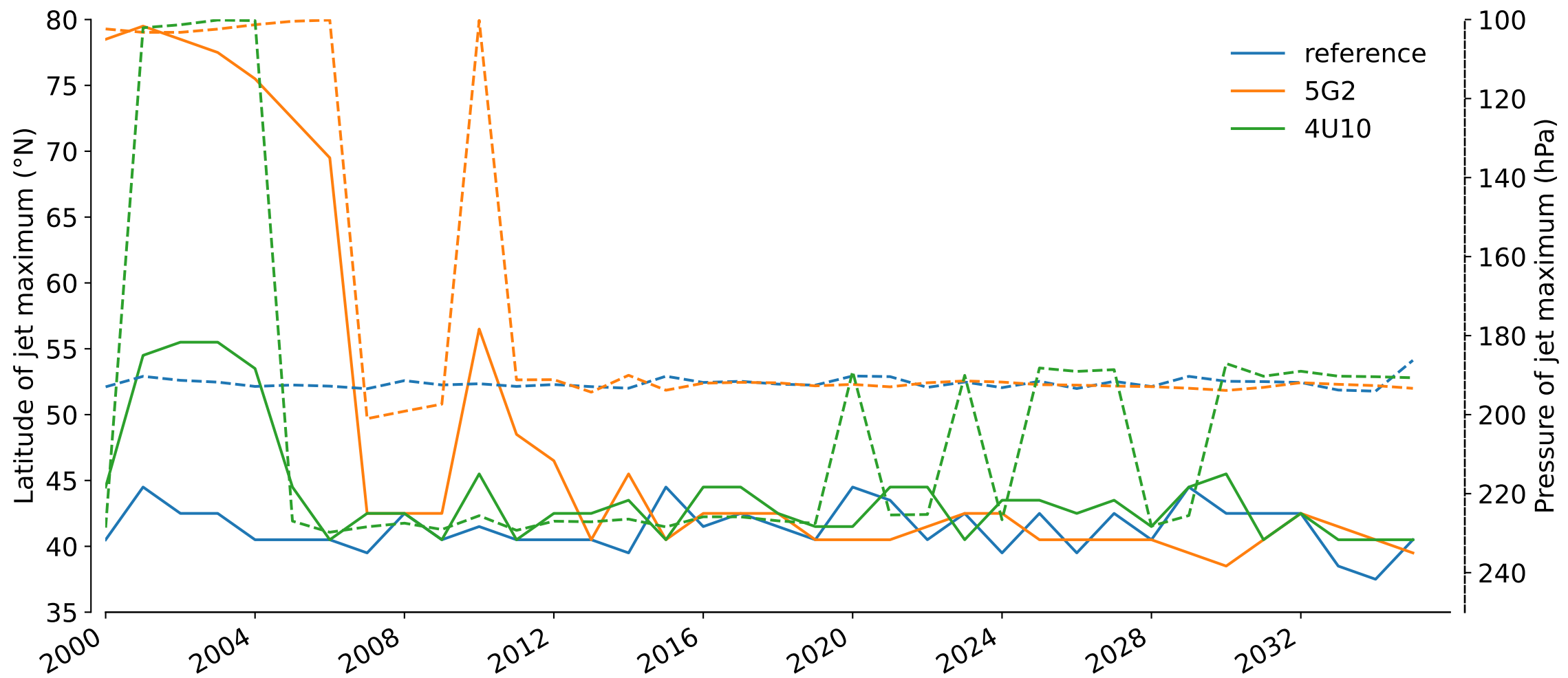
Latitude and pressure of maximum jet wind speed
