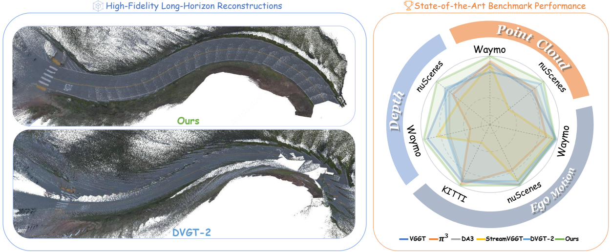
Figure 1 Teaser of Drive3R. Compared with the per-frame streaming baseline DVGT-2 [34], Drive3R reconstructs cleaner and more coherent long-horizon driving scenes with better preserved road geometry. The radar chart further shows state-of-the-art performance across depth, point-cloud, and ego-motion metrics on nuScenes [1], Waymo [15], and KITTI [5].
