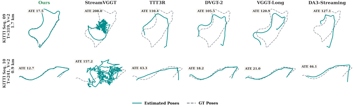
Figure 5 Qualitative trajectory comparison on KITTI [6] sequences 09 and 10. The dashed gray curves denote ground-truth poses, and the solid teal curves denote estimated poses. Our method produces trajectories that are more consistent with the ground truth and obtains lower ATE.
