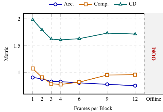
Figure 6 Block-length analysis on nuScenes [2].
