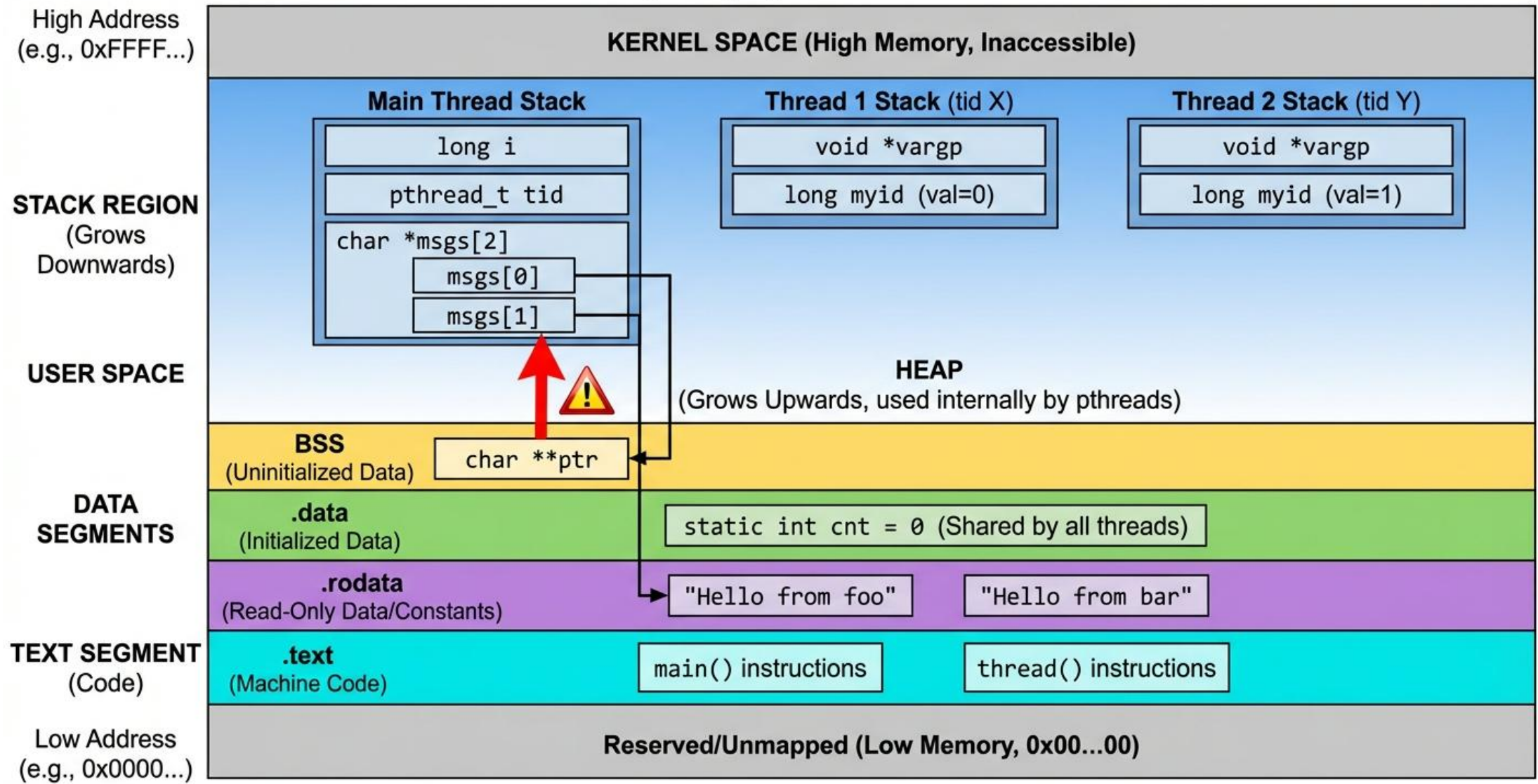
Virtual Memory Map: pthreads & Variable Locations
