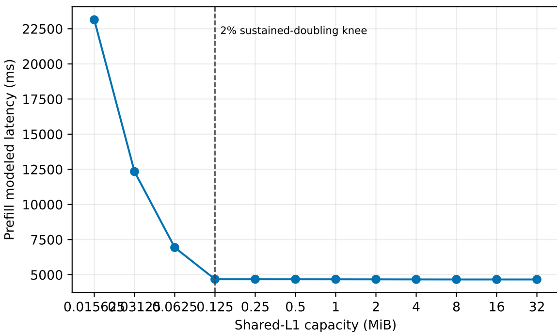
Shared-L1 capacity: one-dimensional analytical sensitivity
