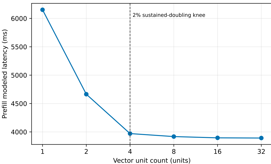
Vector unit count: one-dimensional analytical sensitivity
