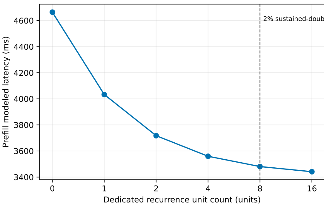
Dedicated recurrence unit count: one-dimensional analytical sensitivity
