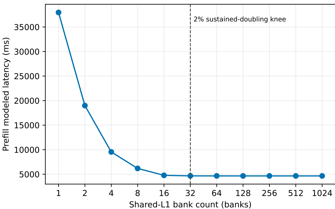
Shared-L1 bank count: one-dimensional analytical sensitivity
