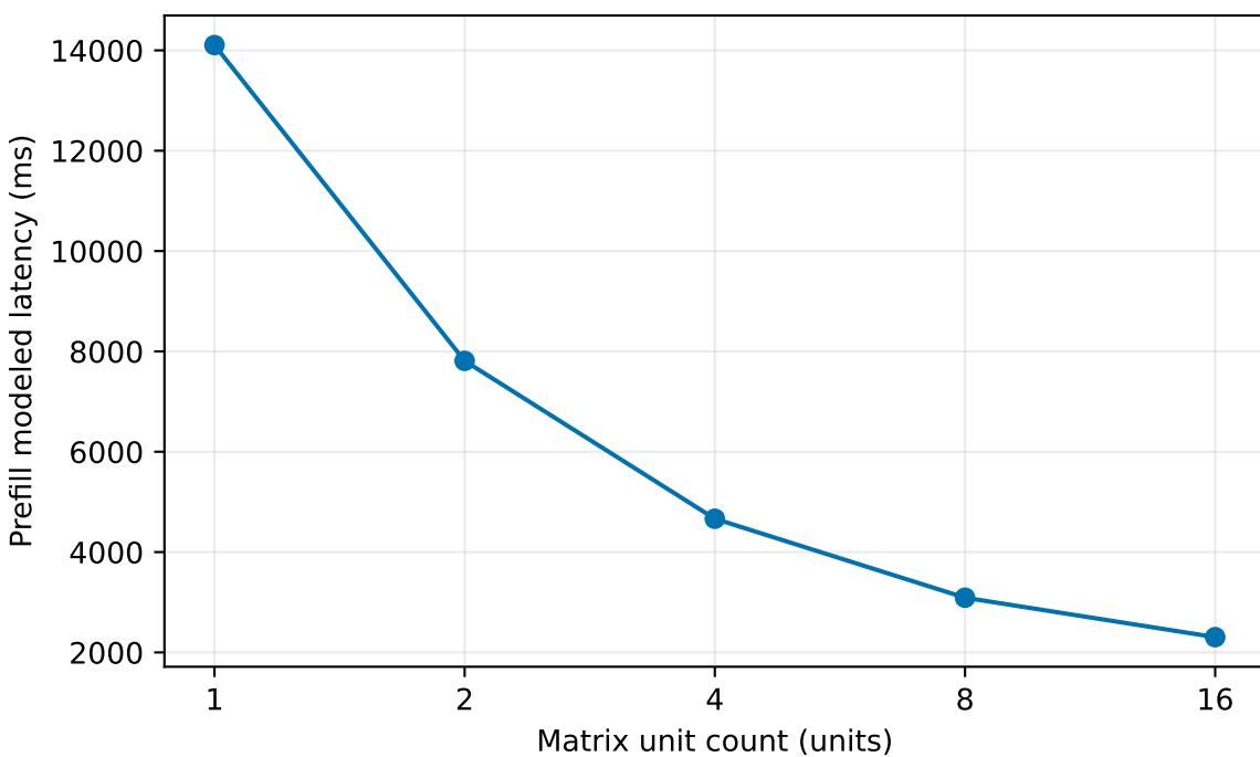
Matrix unit count: one-dimensional analytical sensitivity
