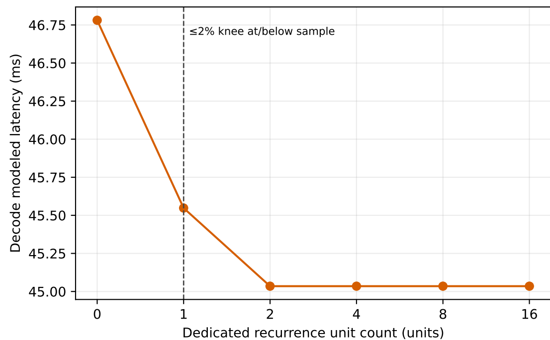
Dedicated recurrence unit count: one-dimensional analytical sensitivity
