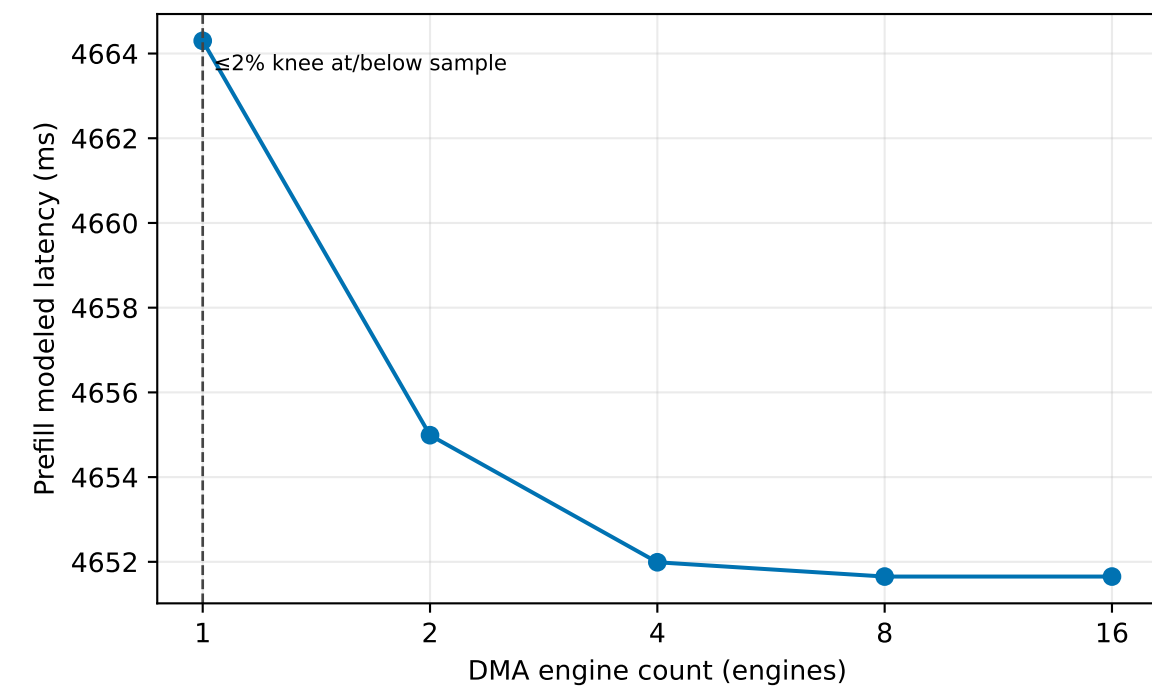
DMA engine count: one-dimensional analytical sensitivity
