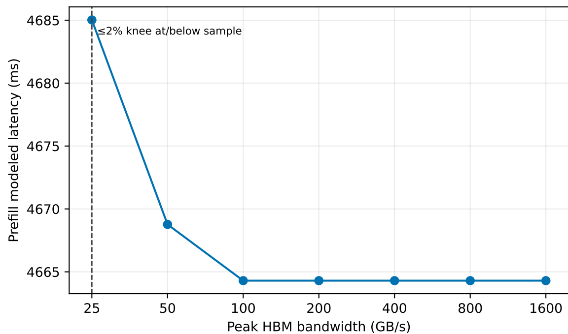
Peak HBM bandwidth: one-dimensional analytical sensitivity
