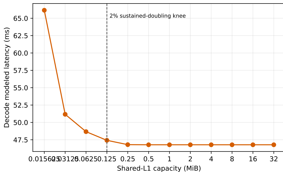
Shared-L1 capacity: one-dimensional analytical sensitivity
