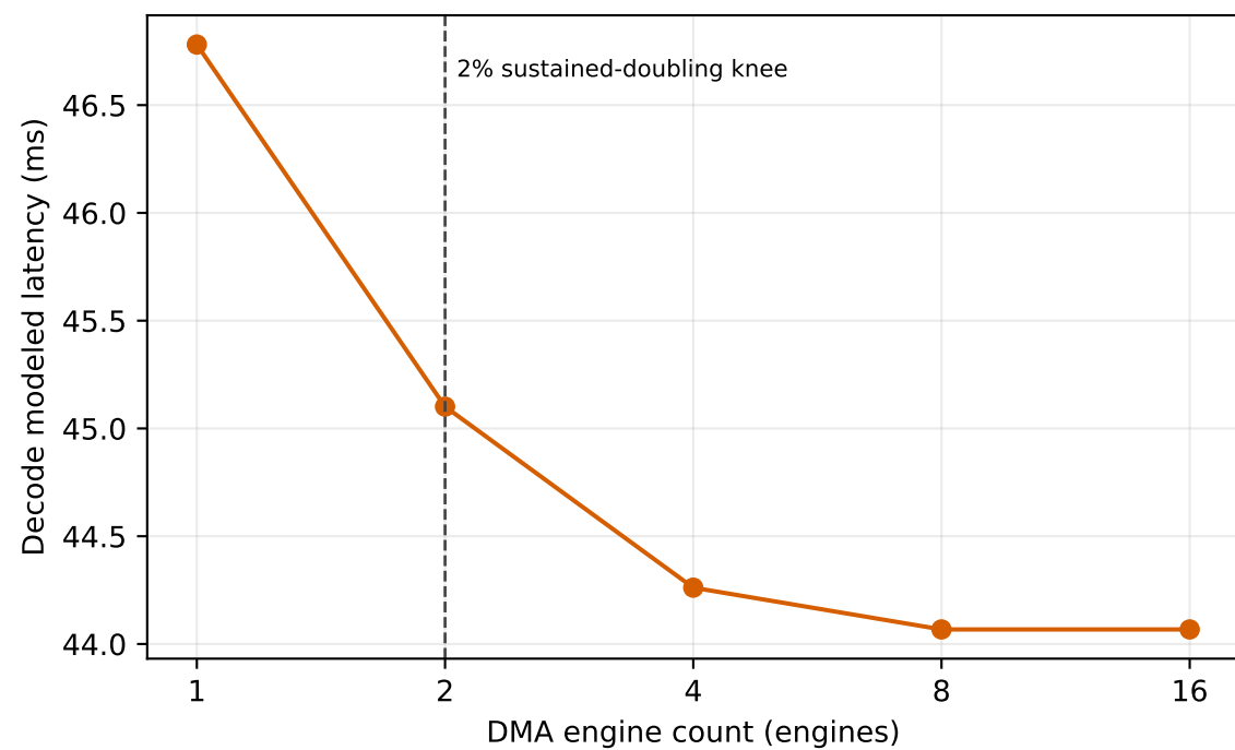
DMA engine count: one-dimensional analytical sensitivity
