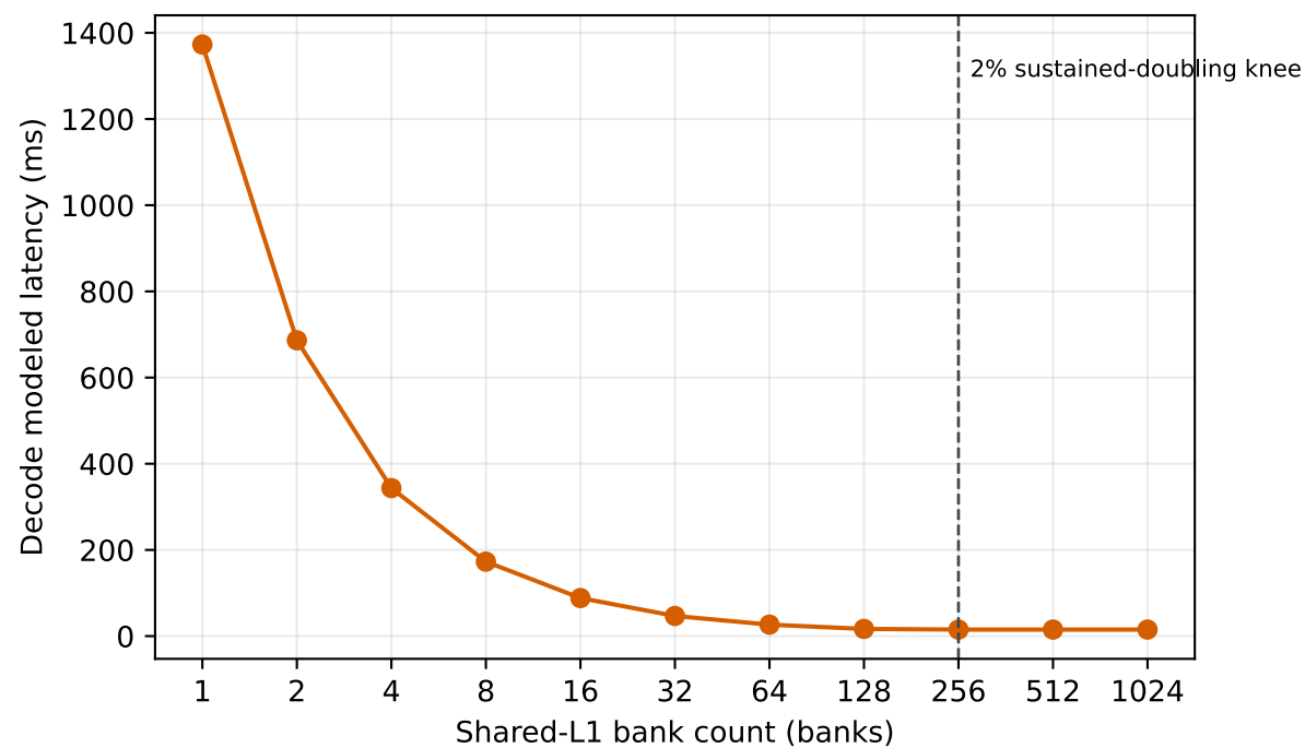
Shared-L1 bank count: one-dimensional analytical sensitivity
