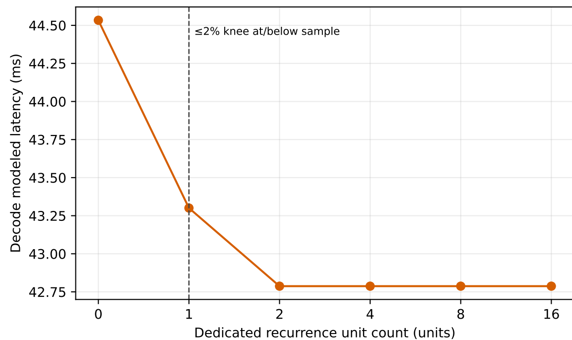
Dedicated recurrence unit count: one-dimensional analytical sensitivity
