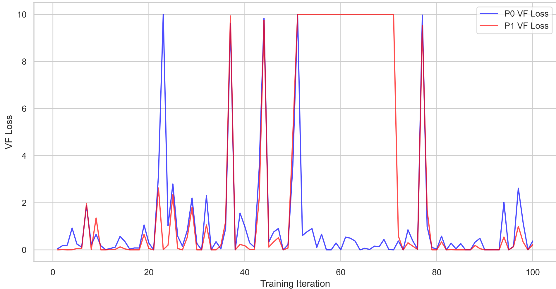
Value Function Loss per Agent
