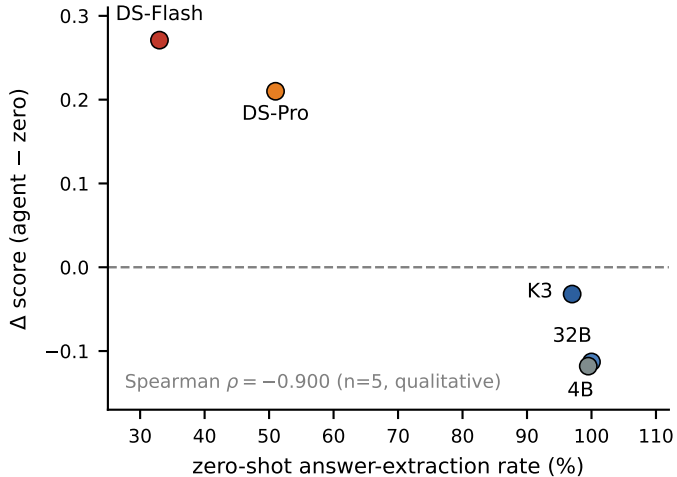
Pathogenesis task
