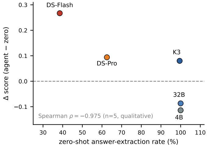
Syndrome task
