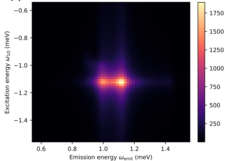
Total rephasing response
