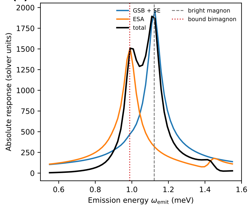
Cut at \omega_{1Q} = -1.126 meV
