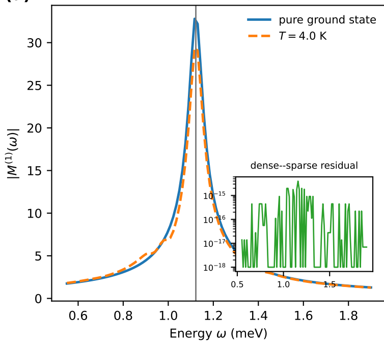
Total rephasing response
