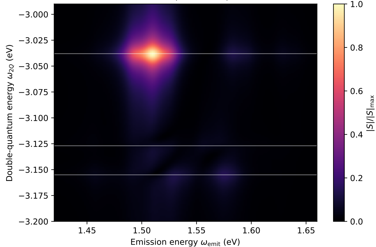
Fifth-order 2Q spectrum, \eta = 8 meV
