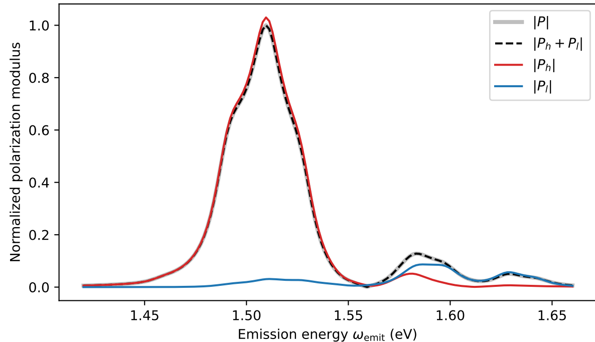
Mode-resolved detection at \omega_{2Q} = -E_1
