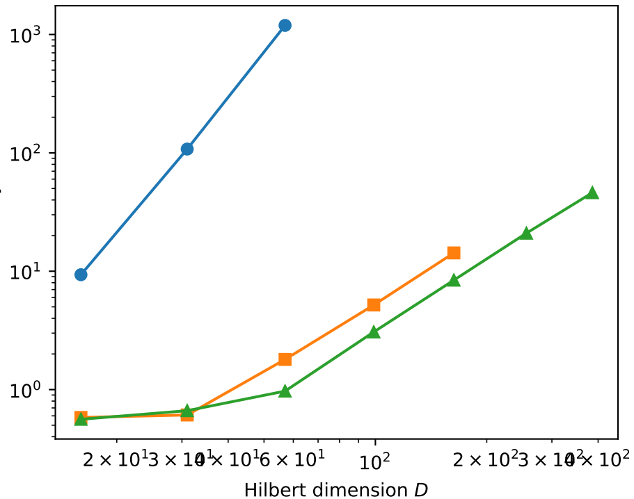
Peak memory (MB)
