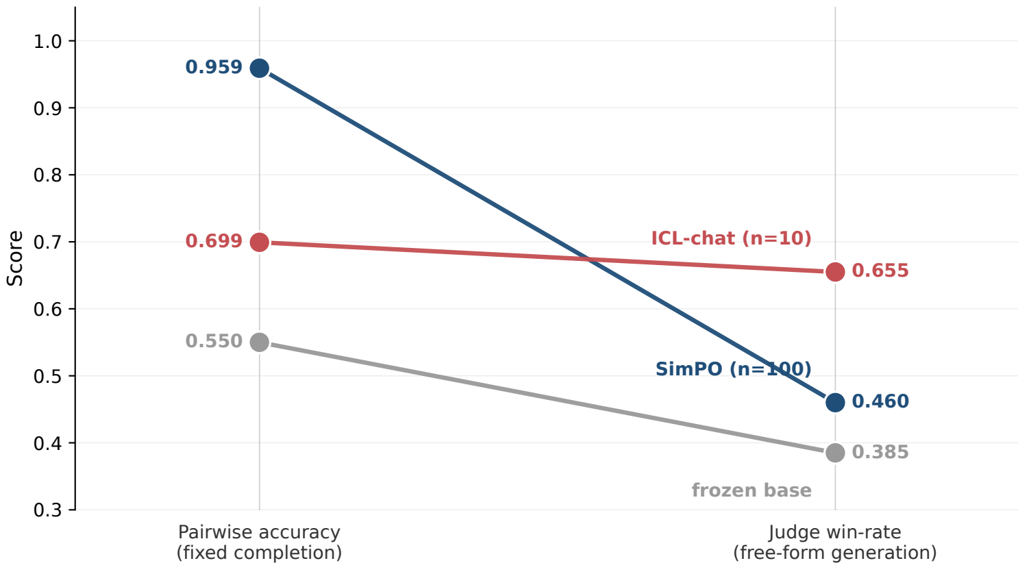
Same models, different evaluation format — the ranking inverts
