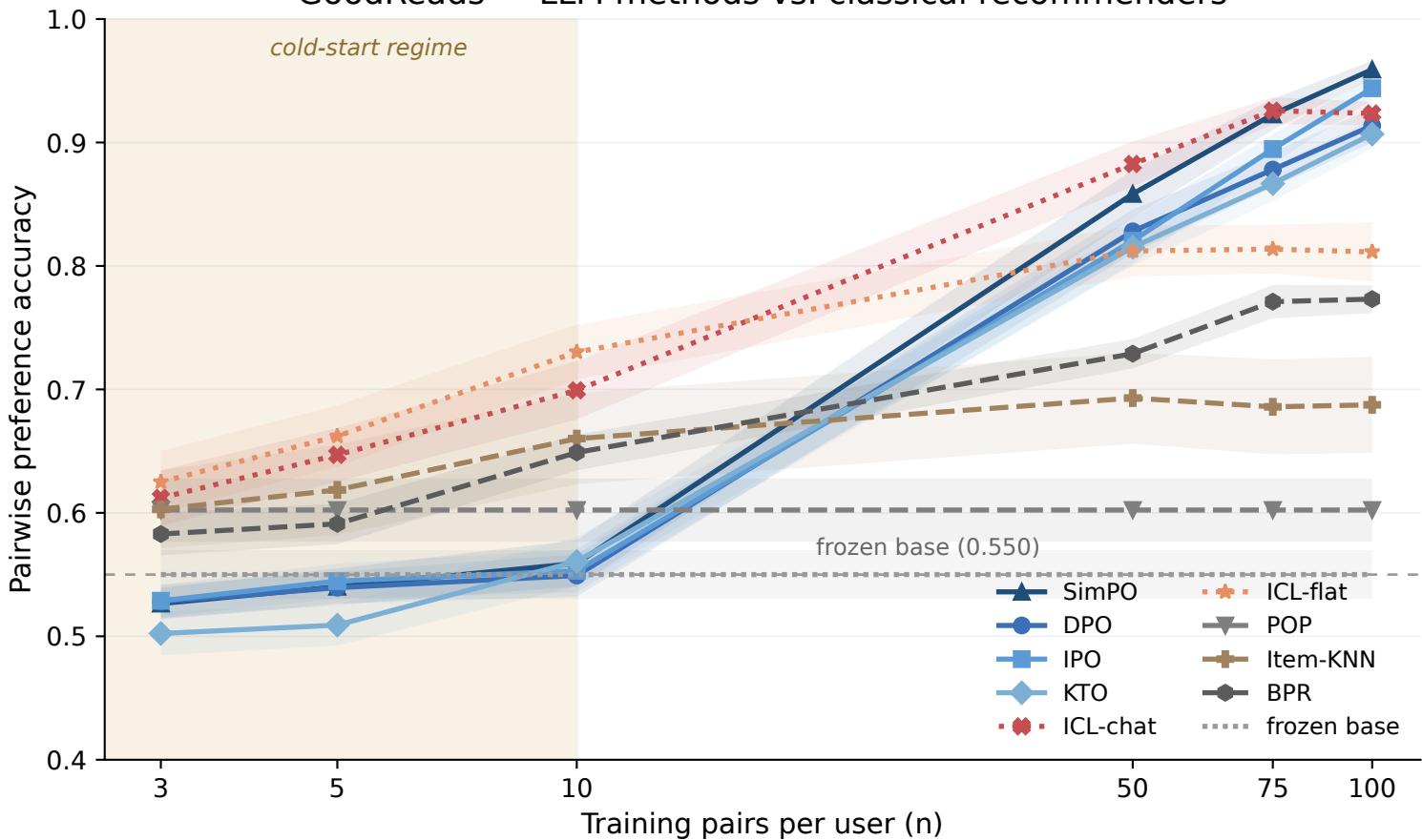
GoodReads — LLM methods vs. classical recommenders
