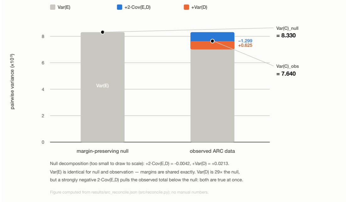
Figure 4: The exact decomposition \text{Var}(C) = \text{Var}(E) + 2\text{Cov}(E, D) + \text{Var}(D) on ARC. \text{Var}(E) is identical for null and observation by construction; the observed column's negative covariance term outweighs its 29\times -inflated variance term, landing below the null.
