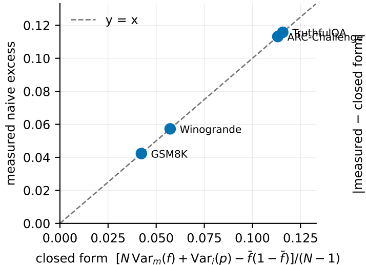
a Lemma 2 predicts the reported excess exactly
