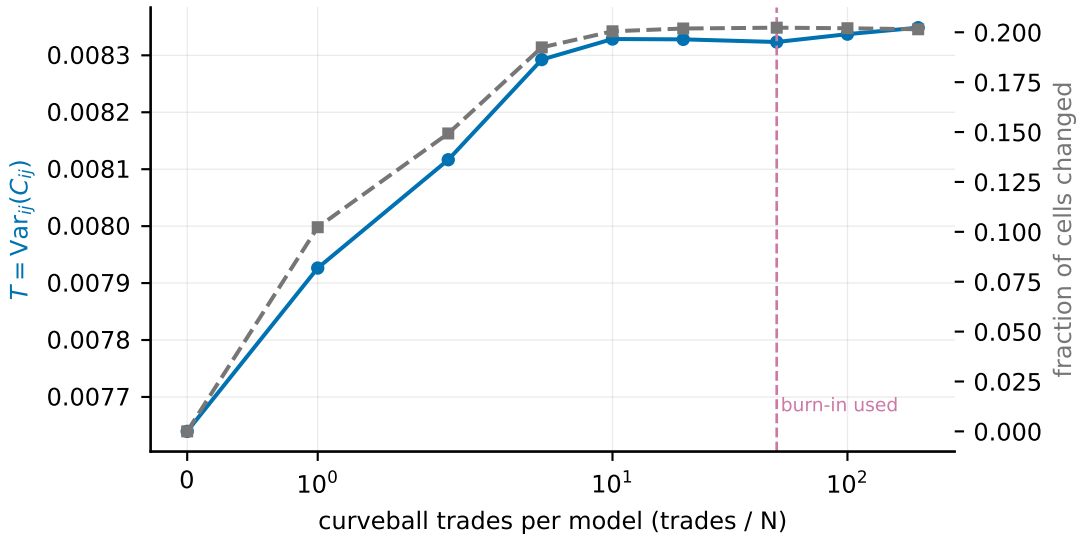
Chain reaches its plateau by ~10 trades/N
