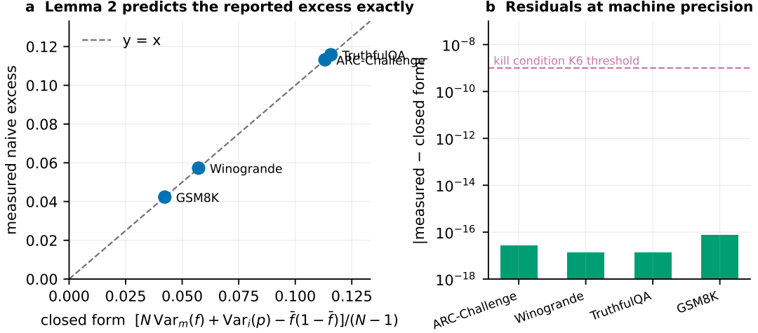
Figure 1: Lemma 2 predicts the measured excess exactly on all four benchmarks (panel a); the residual sits at machine precision, well below the 10^{-9} validation threshold set in the pre-registration (panel b).
