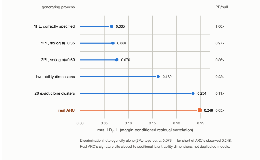
Fig. 3 Identification evidence: real ARC's residual correlation (orange) sits far beyond what two-parameter discrimination heterogeneity alone can produce, and its \lambda_1^2 / \sum \lambda^2 signature (Table 4) matches a multi-ability structure rather than duplicated models.
