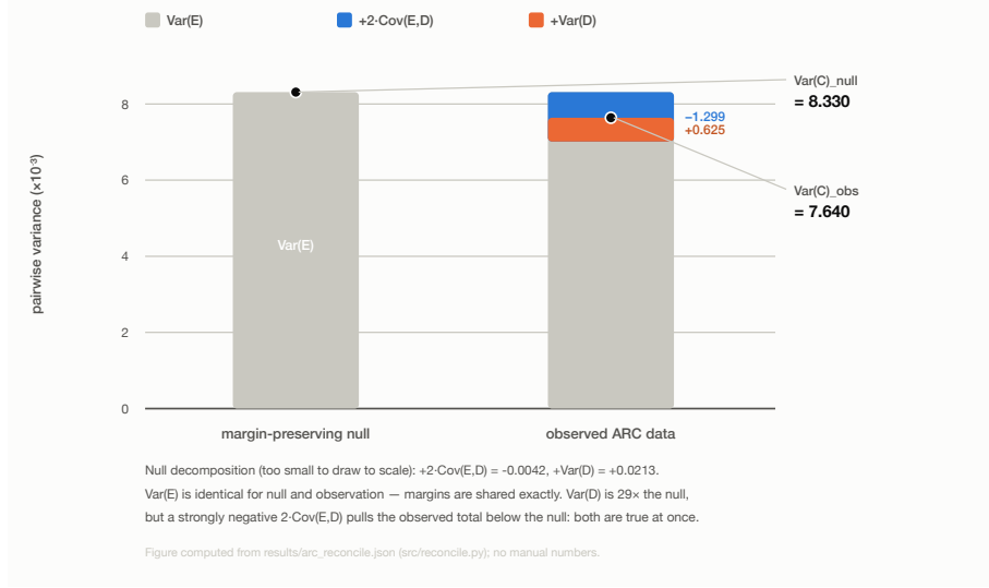
Fig. 4 The exact decomposition \text{Var}(C) = \text{Var}(E) + 2\text{Cov}(E, D) + \text{Var}(D) on ARC. \text{Var}(E) is identical for null and observation by construction; the observed column’s negative covariance term outweighs its 29×-inflated variance term, landing below the null.
