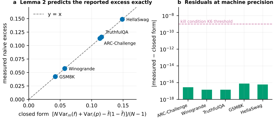
Fig. 1 Lemma 2 predicts the measured excess exactly on all five benchmarks (panel a); the residual sits at machine precision, well below the 10^{-9} validation threshold set in the pre-registration (panel b).
