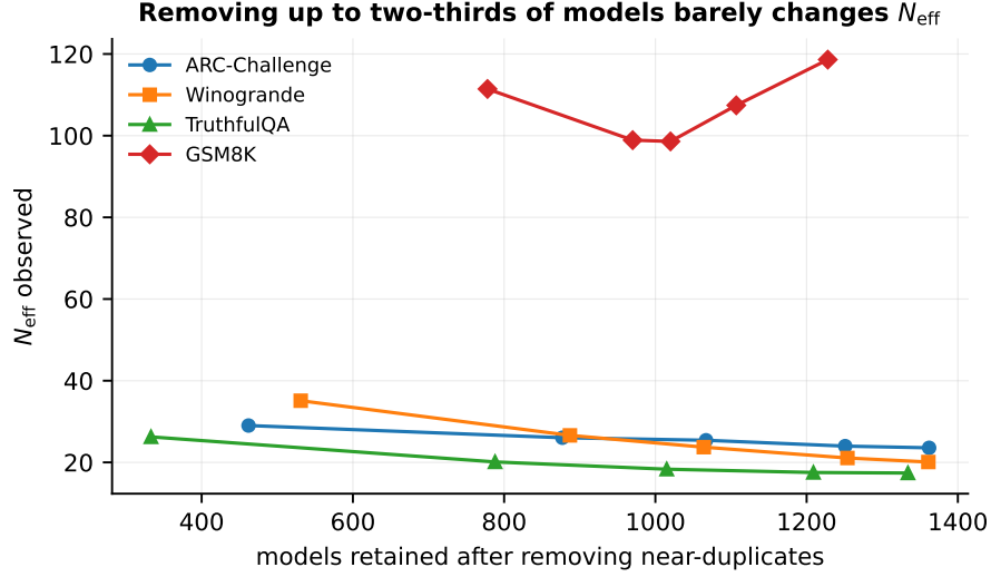
Fig. 5 Observed participation ratio as near-duplicate models (agreement \geq threshold, one representative kept per cluster) are progressively removed. Removing up to two-thirds of each benchmark’s models moves the statistic by only a few units.
