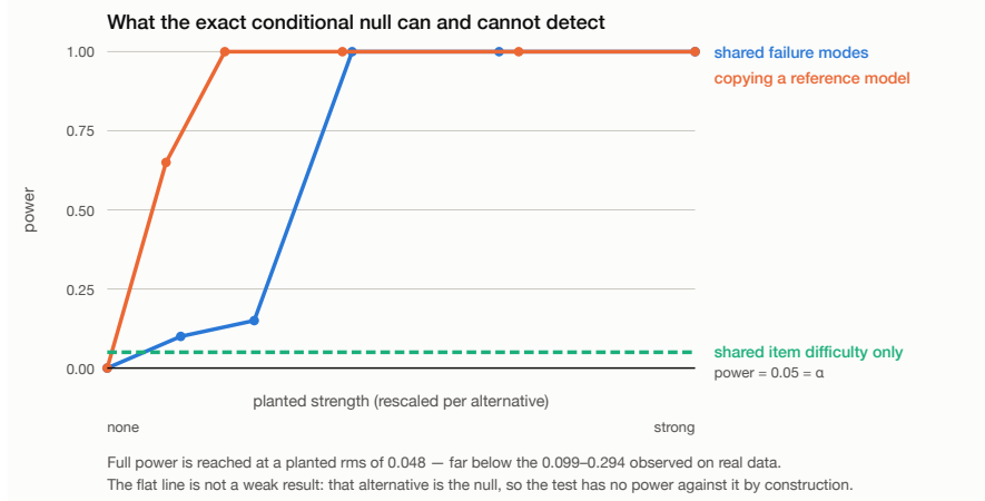
Fig. 6 Detection power against three planted alternatives ( results/power_study.json ). The dashed line is the design’s blind spot rather than a weak result: a population in which every model shares one item-difficulty profile and differs only in overall ability is exactly what the null describes, so no test conditioning on the item margins can separate it from chance.
