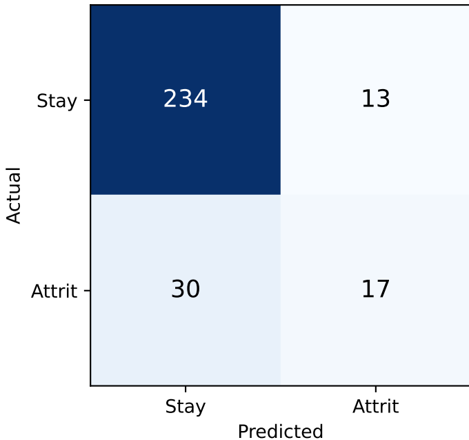
Confusion matrix (holdout, thr=0.50)
