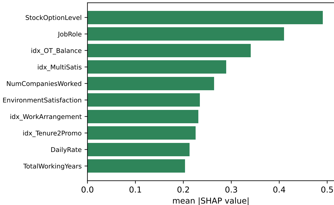
SHAP feature importance (holdout)
