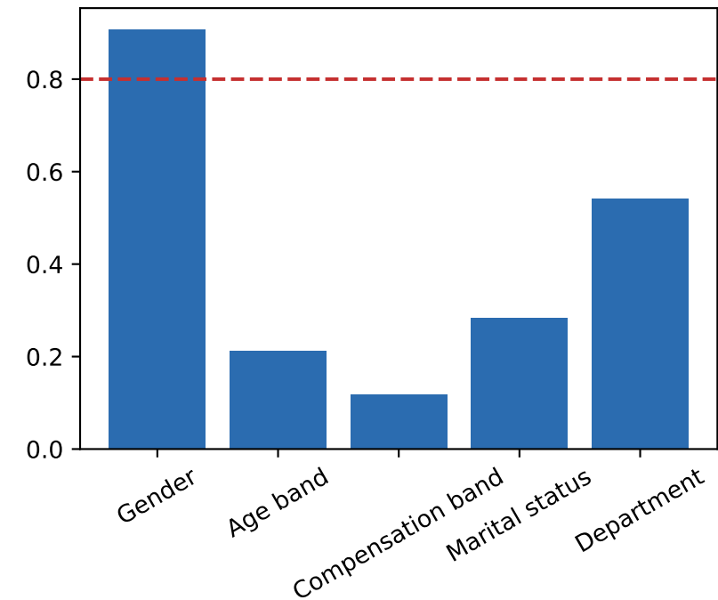
Disparate-impact ratio
