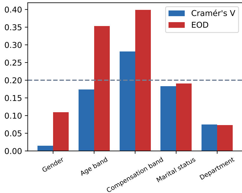
Cramér's V &amp; EOD
