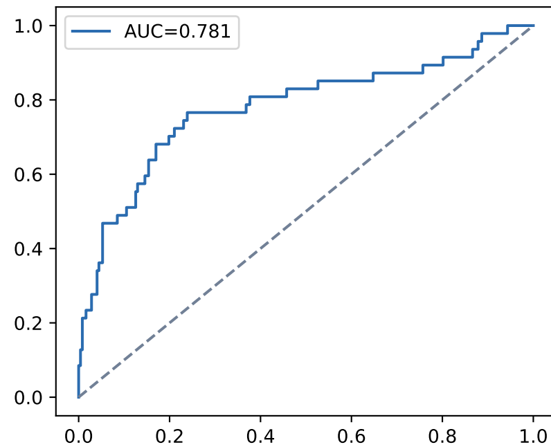
(a) ROC
