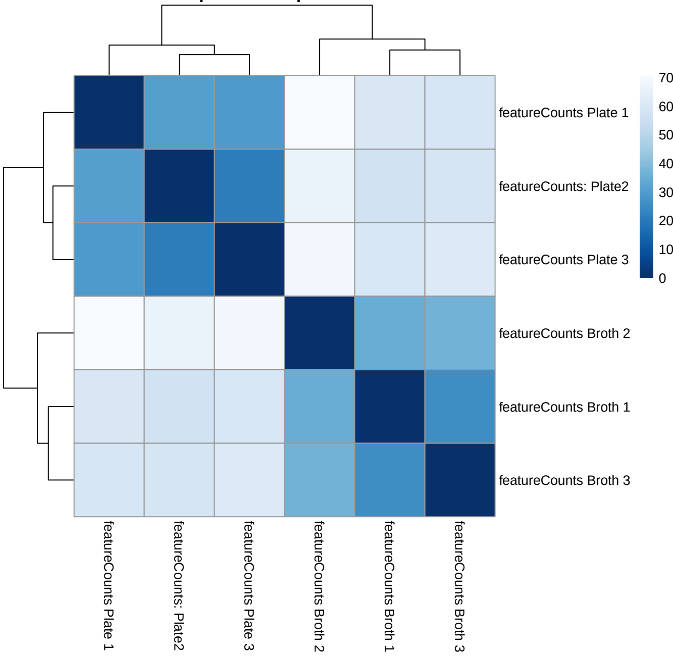
Sample-to-sample distances
