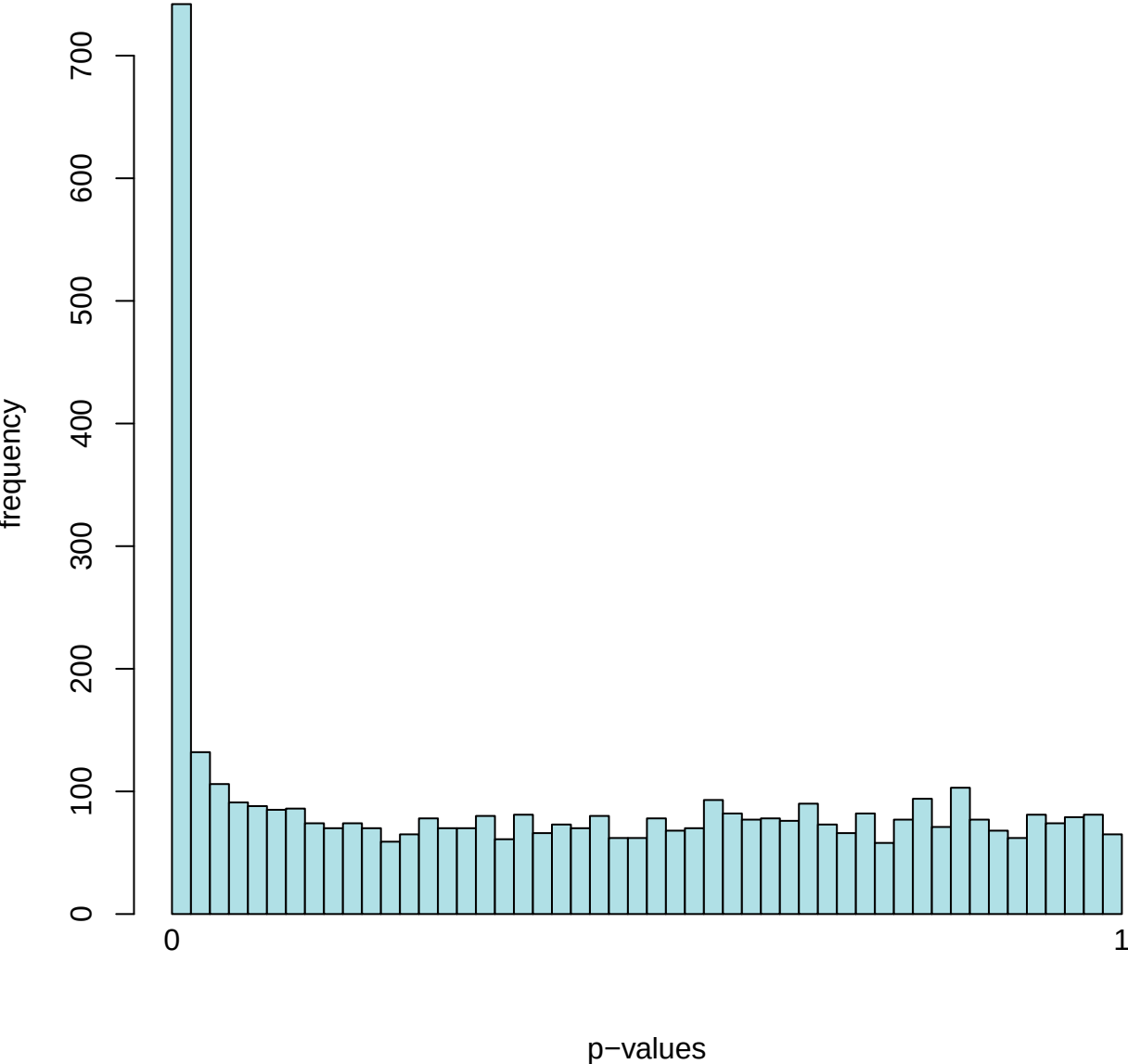
Histogram of p-values for Growth_Media: Wildtype vs egtBmutant
