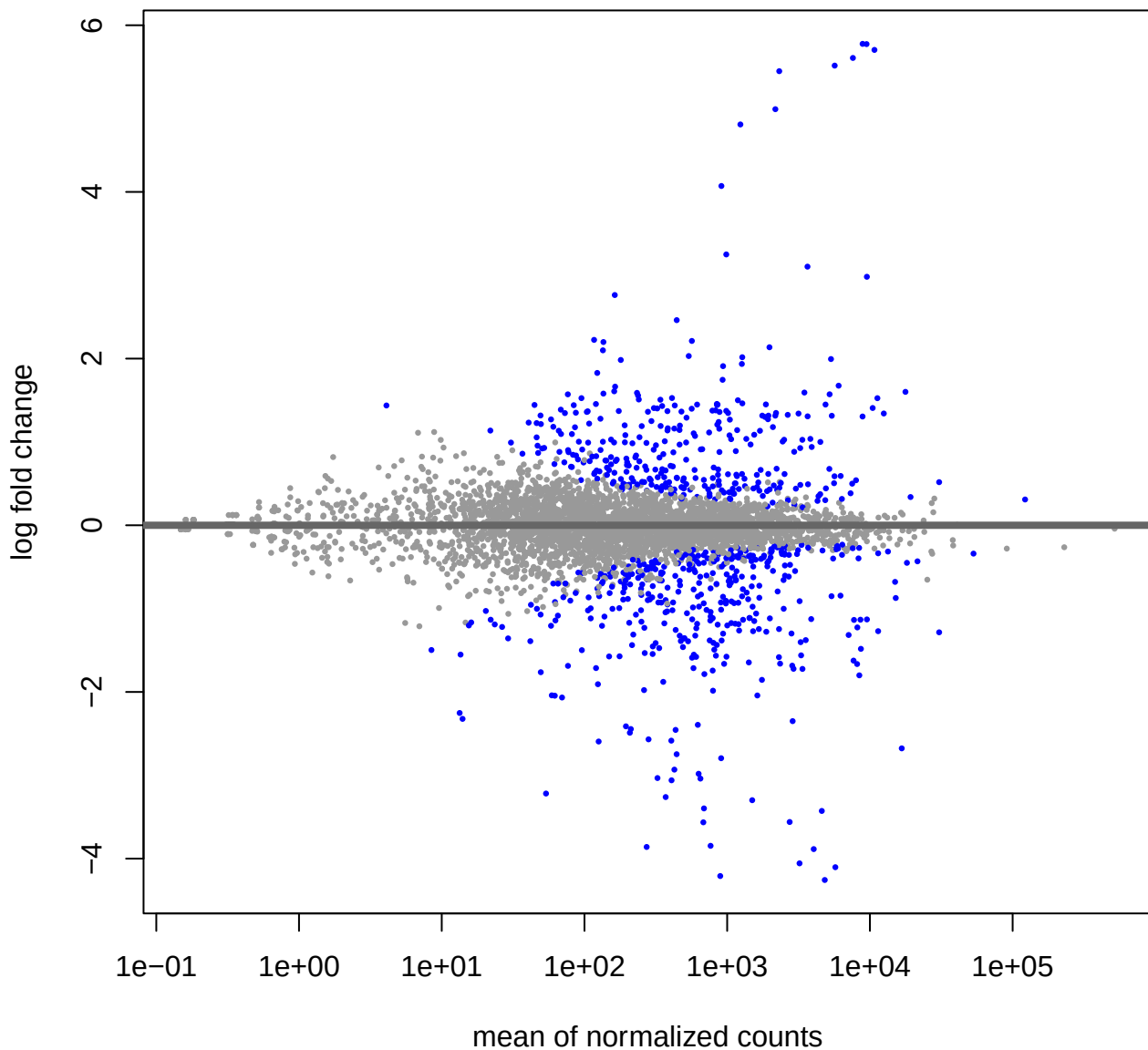
MA-plot for Growth_Media: Wildtype vs egtBmutant
